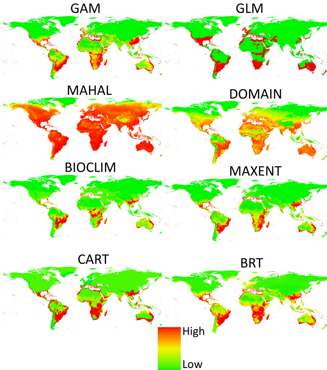
Figure S4: Predicted probability of occurrence for each model type under current climate conditions. Notice that DOMAIN and MAHAL produce much higher probabilities in large areas where the other models are more conservative, systematically over-predicting the potential range of the species.
