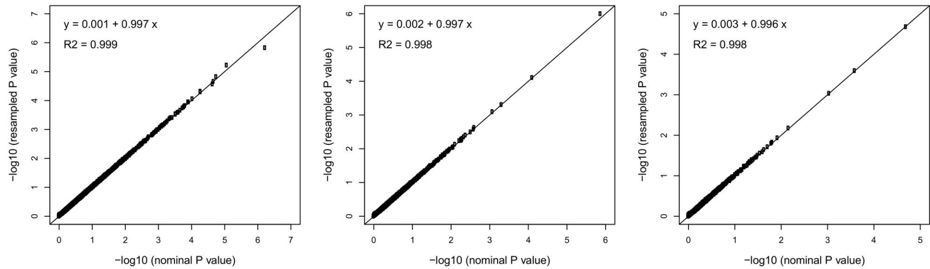
Figure S1. Nominal versus resampling P value for different trait variants. Left panel: the original trait; central panel: GRAMMAR+ trait transformation; right panel: environmental residuals. The number of resampling was set as 1000/(P \text{ value}) with upper limit of 10^6 .
