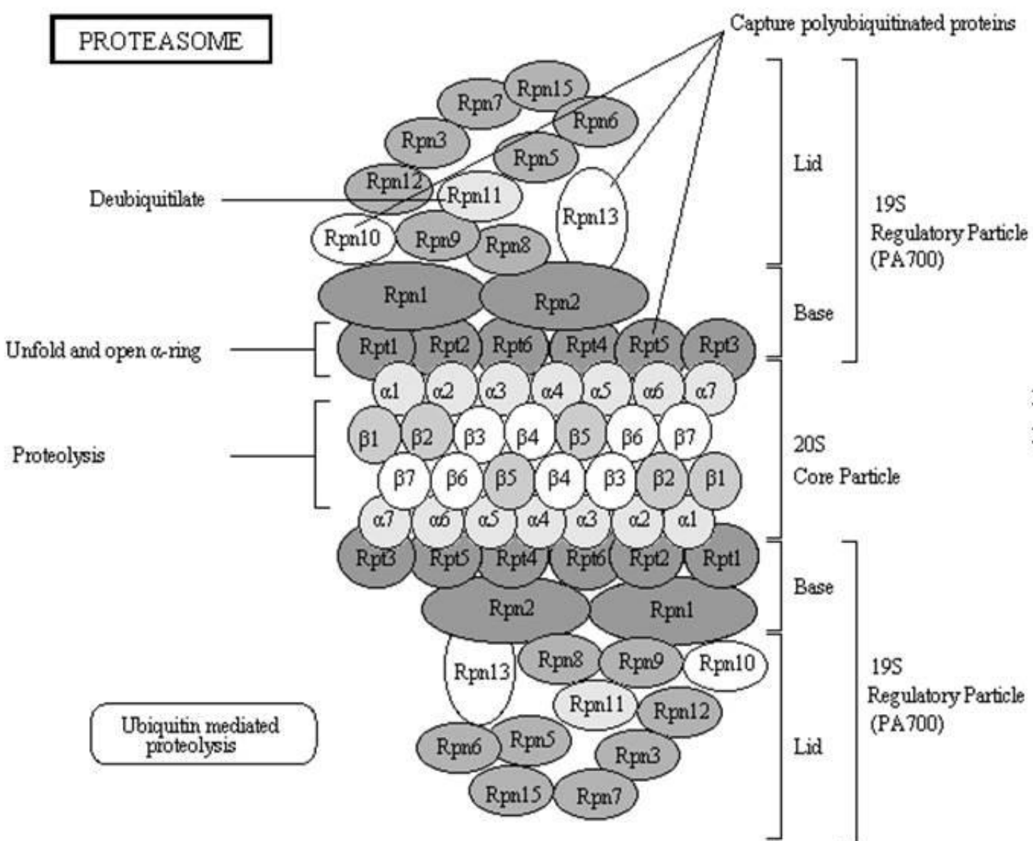
PA700-20S-PA700 (26S proteasome)
