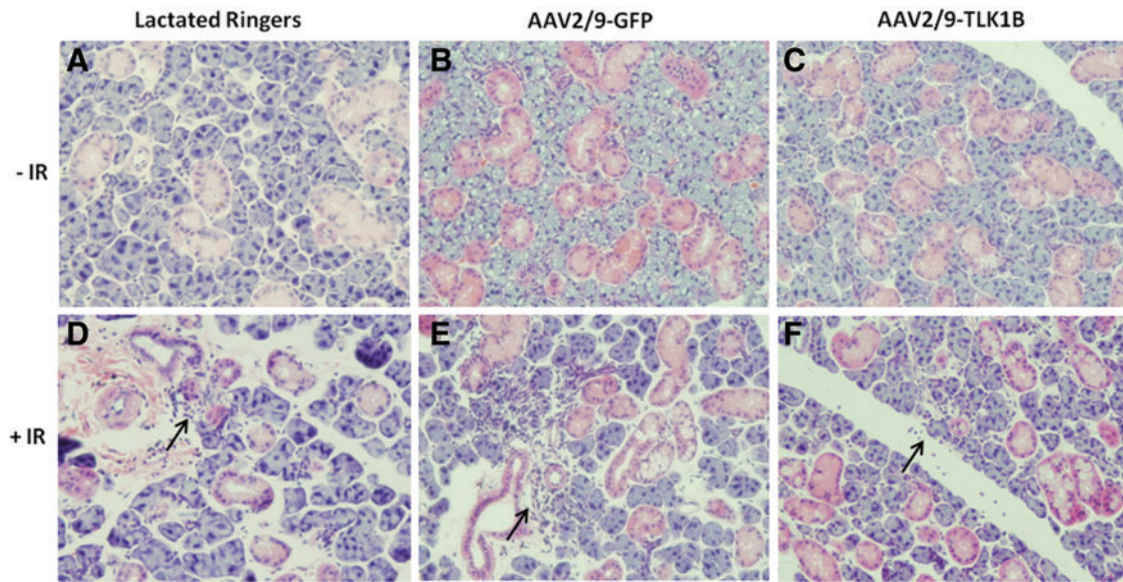
SUPPLEMENTARY FIG. S3. Histopathological manifestations after irradiation. Hematoxylin and eosin stain of salivary gland secretions pretreated with (A and D) lactated Ringers, (B and E) AAV9-GFP, and (C and F) AAV9-TLK1B. (A–C) Nonirradiated (–IR) glands. (D–F) Eight weeks after completion of radiation (+IR). Arrows point to inflammatory infiltrate. +IR, radiated; –IR, nonirradiated. Magnification, 200 \times .
