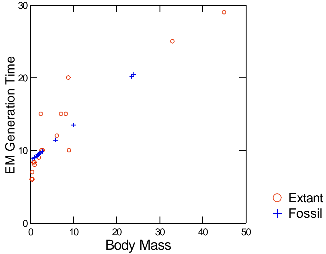
Figure S7 EM fit. Plot showing body mass and generation time for extant species (red symbols), and body mass and imputed generation time for fossil taxa (blue symbols) using a EM fit.
