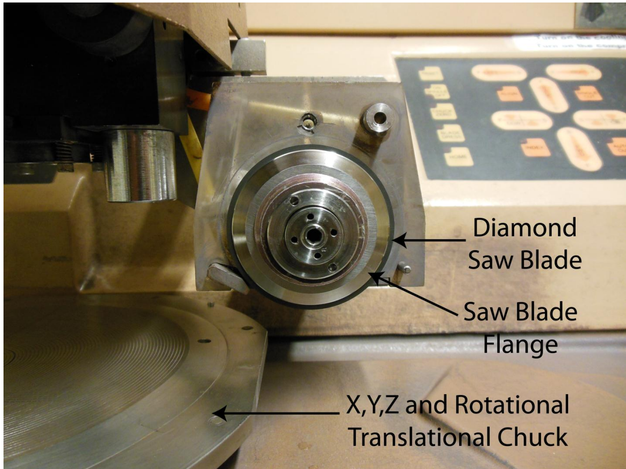
Fig. S2 Close-up of the micro-dicing saw. The diamond saw blade is held by compression in the saw blade flange. When cuts are made the blade assembly remains fixed while the x, y, z, and rotational translation chuck performs the necessary movements to accomplish the desired cuts.
