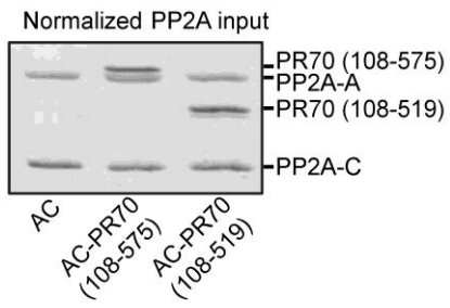
Figure S2. Related to Figure 5. Normalized input of PP2A AC core enzyme, AC-PR70 (108-575) holoenzyme, and AC-PR70 (108-519) holoenzyme for phosphatase assay in Figure 5B&C was examined by SDS-PAGE and visualized by Coomassie blue staining.
