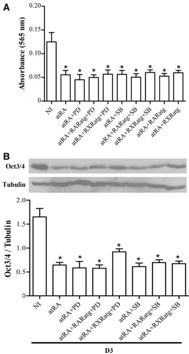
SUPPLEMENTARY FIG. S3. Cell proliferation ( A ) and Oct3/4 protein expression ( B ) in cultures treated with combinations of atRA, RAR/RXRatg, and MAPK inhibitors. Analysis was done as indicated in the legend to Fig. 2. Values are expressed as the means \pm SEM of three independent cell series, and *indicates a significant difference compared with the NI condition ( P < 0.05 ).
