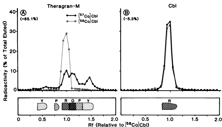
FIGURE 1 Paper chromatograms of Ⓞ Cbl isolated from a multivitamin-mineral pill (Theragra-M, ferrous carbonate form) and Ⓞ crystalline CN-Cbl. Ⓞ, the sample was obtained from the supernatant of an homogenate (Methods) of 100 Theragra-M pills, stated to contain a total of 367 nmol of CN-Cbl, which was incubated with 2 pmol of CN-[ 57 Co]Cbl for 2 h at 37°C. The Cbl was then isolated using reverse affinity chromatography on R protein-Sepharose followed by phenol extraction as described under Methods. The recovery of [ 57 Co]Cbl was 61.3%. CN-[ 58 Co]Cbl, 10 pmol, was added to the purified Cbl immediately before paper chromatography. Ⓞ, the sample contained 200 nmol of crystalline CN-Cbl, 1 pmol of CN-[ 57 Co]Cbl and 10 pmol CN-[ 58 Co]Cbl, all of which were combined immediately before paper chromatography. Paper chromatography was performed in solvent I as described under Methods. Paper chromatograms were examined for the presence of colored spots (Y, yellow; P, pink; R, red; O, orange) and then cut into 38 equal fractions, which were assayed for 57 Co and 58 Co. The numbers in parentheses indicate the amounts of [ 57 Co]Cbl present as Cbl analogues, relative to that of [ 58 Co]Cbl, and were calculated as described under Methods.
