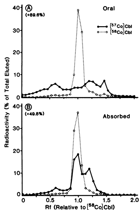
FIGURE 5 Gastrointestinal absorption of ^{57}\text{Co} Cbl analogues from a multivitamin-mineral pill (Theragra-M, ferrous carbonate form). \odot paper chromatogram of CN- ^{57}\text{Co} Cbl that was incubated with an aqueous extract of Theragra-M for 2 h at 37°C and immediately given orally to mice, (~2 pmol of total ^{57}\text{Co} Cbl per mouse). \ominus , paper chromatogram of the same ^{57}\text{Co} Cbl that was extracted from mouse tissues 24 h after its oral administration. Additional details concerning the preparation of the Cbl analogues and the performance of paper chromatography are described in the legend to Fig. 1A and under Methods.
