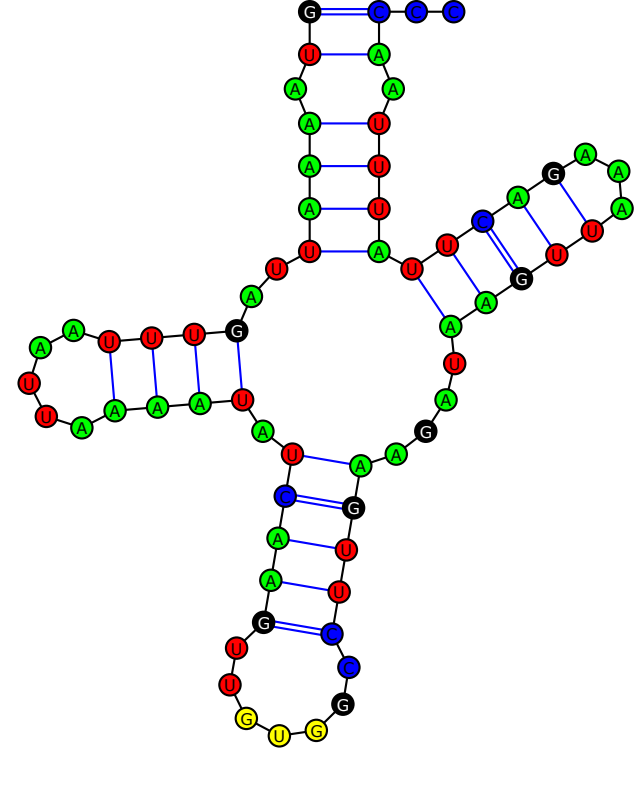
tRNA-His(GUG)
