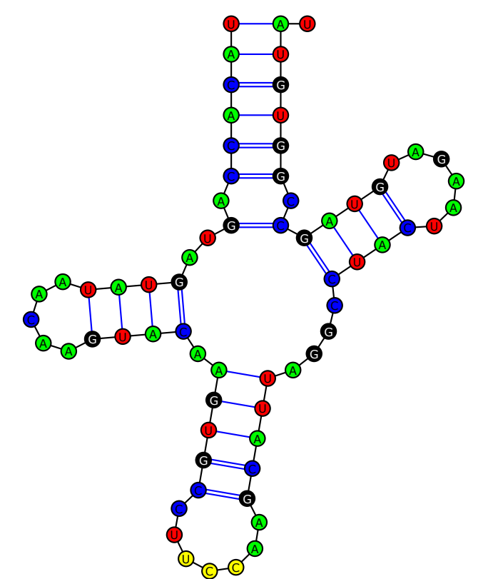
tRNA-Gly(UCC)
