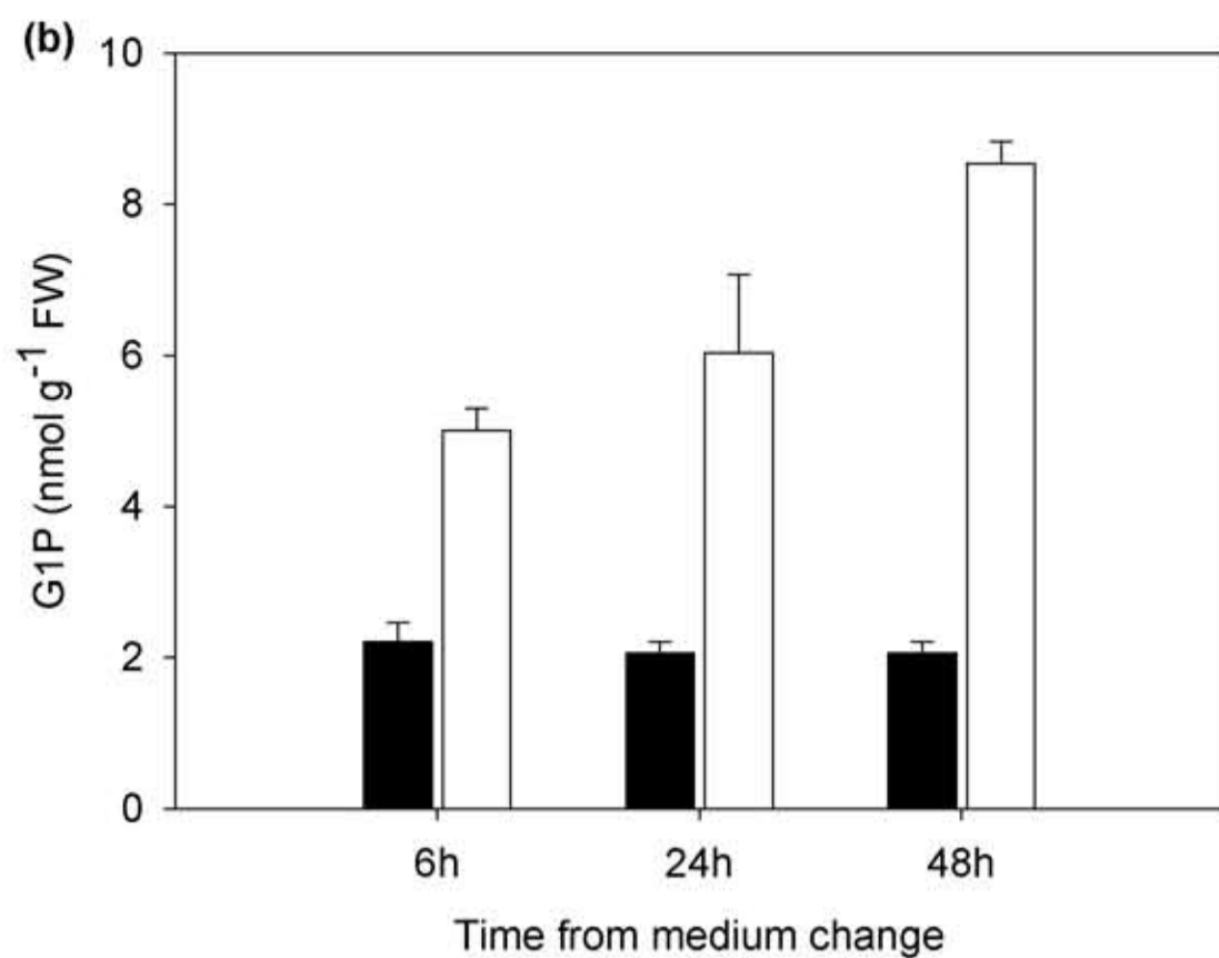
Supplementary Fig. 1 G6P and G1P accumulation in response to glucose feeding. (a), G6P and (b), G1P compared to the starvation control. Data are averages with standard deviations of 3 independent samples.
