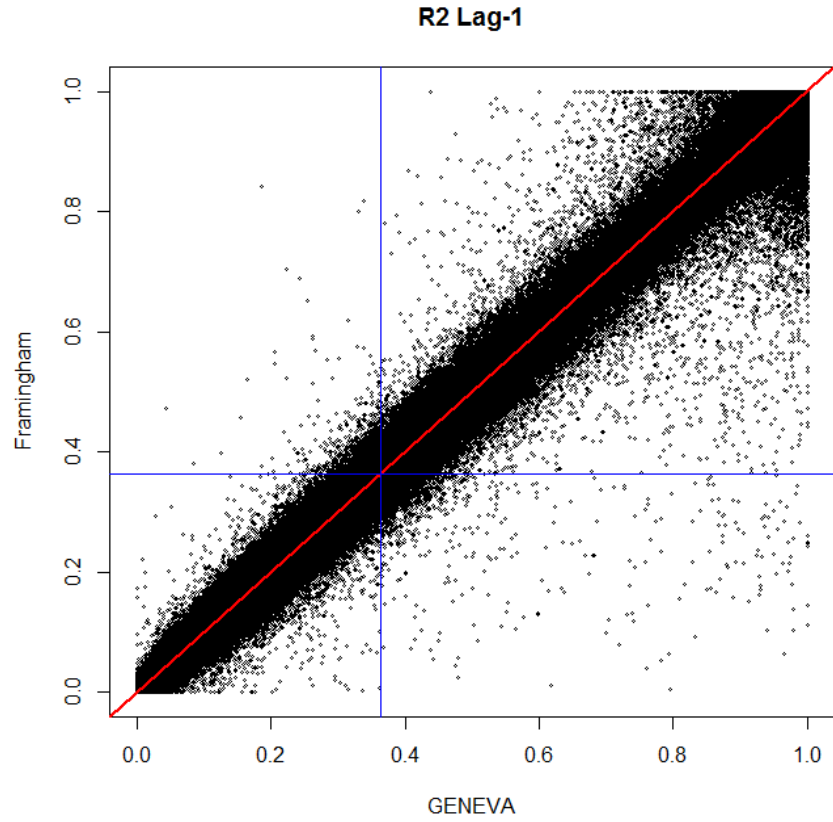
Figure S1. Squared-correlation between genotypes at adjacent markers observed in the FHS (vertical axis) and GEN datasets. The average inter-marker distance in the platform was 7.2kb The blue lines gives the median squared-correlation in both datasets.
