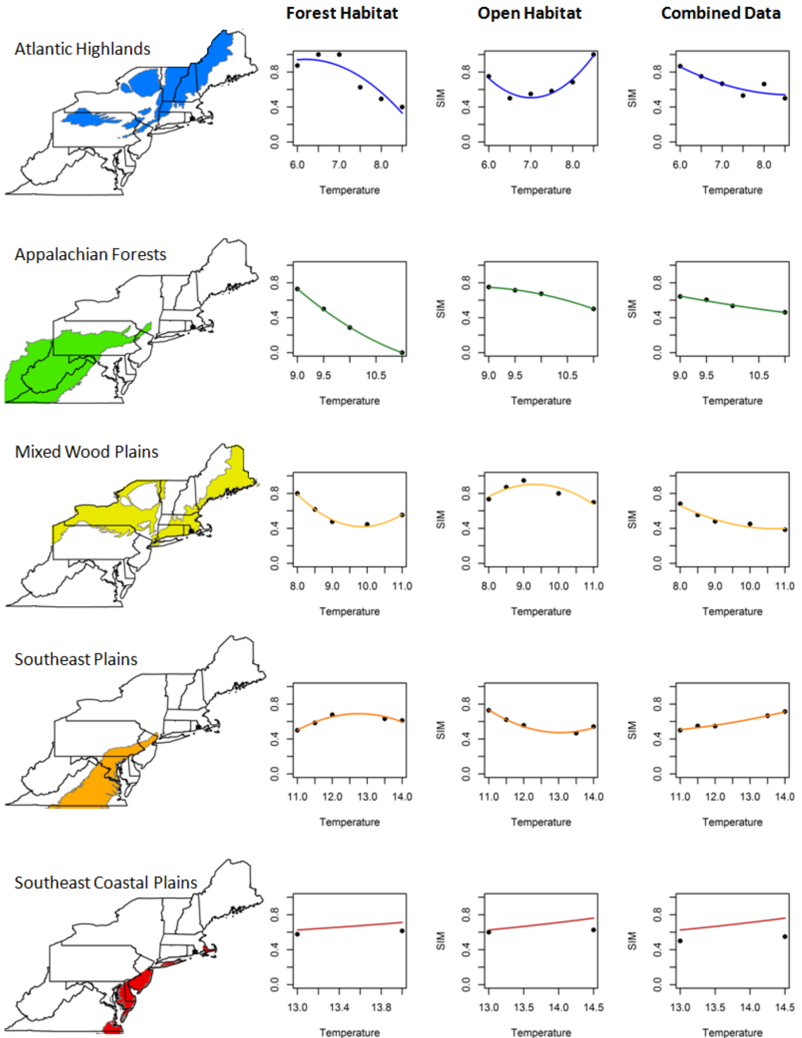
File S6 Figure S9: Beta SIM vs. Temperature regressions subdivided by ecoregion and habitat type
