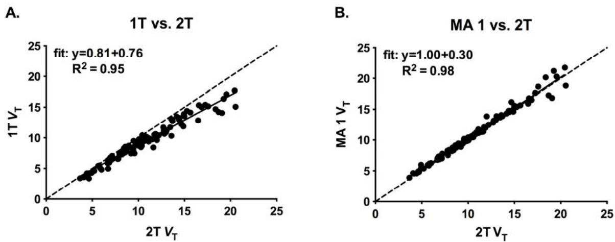
Suppl. Fig. 1. Model comparison of 1T and MA1 vs. 2T for [ ^{11}\text{C} ]ABP688 V_T for all conditions and ROIs. A) 1T underestimated 2T V_T values and B) MA1 values were in very good agreement with 2T V_T values as indicated with the regression fit (solid line). The identity plot (dashed line) was added for reference. Only V_T estimates with percent standard error <20% were used in these comparisons.
