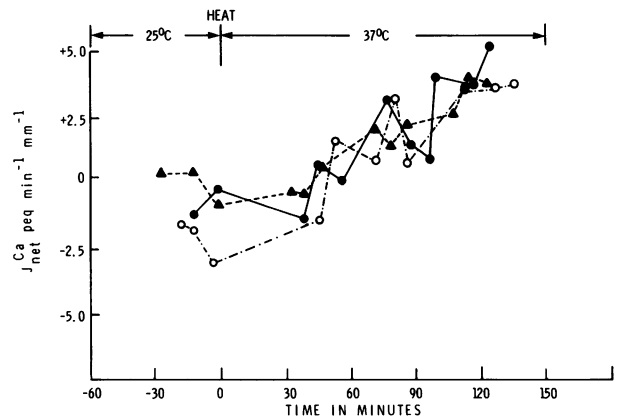
FIGURE 3. The effect of cold and subsequent heating on, J_{net}^{Ca} .
