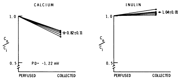
FIGURE 1. The ratio of 45 Ca collected ( C o ) to 45 Ca perfused ( C i ) (left panel), and the ratio of [ 3 H]inulin collected to perfused (right panel), in experiments with perfusate and bath of identical 45 Ca specific activity.
