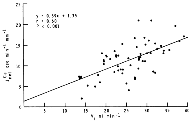
FIGURE 2. The relationship of J_{net}^{Ca} to perfusion rate ( V_i ).
