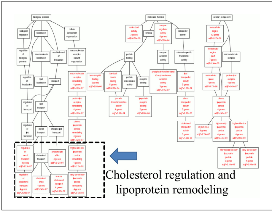
Supplementary Figure 3. Gene Ontology of common proteins in different samplings. Cholesterol regulation and lipoprotein remodeling appeared to be the most significant biological function in which the proteins participate. The figure was constructed using WebGestalt web-tool [24].
