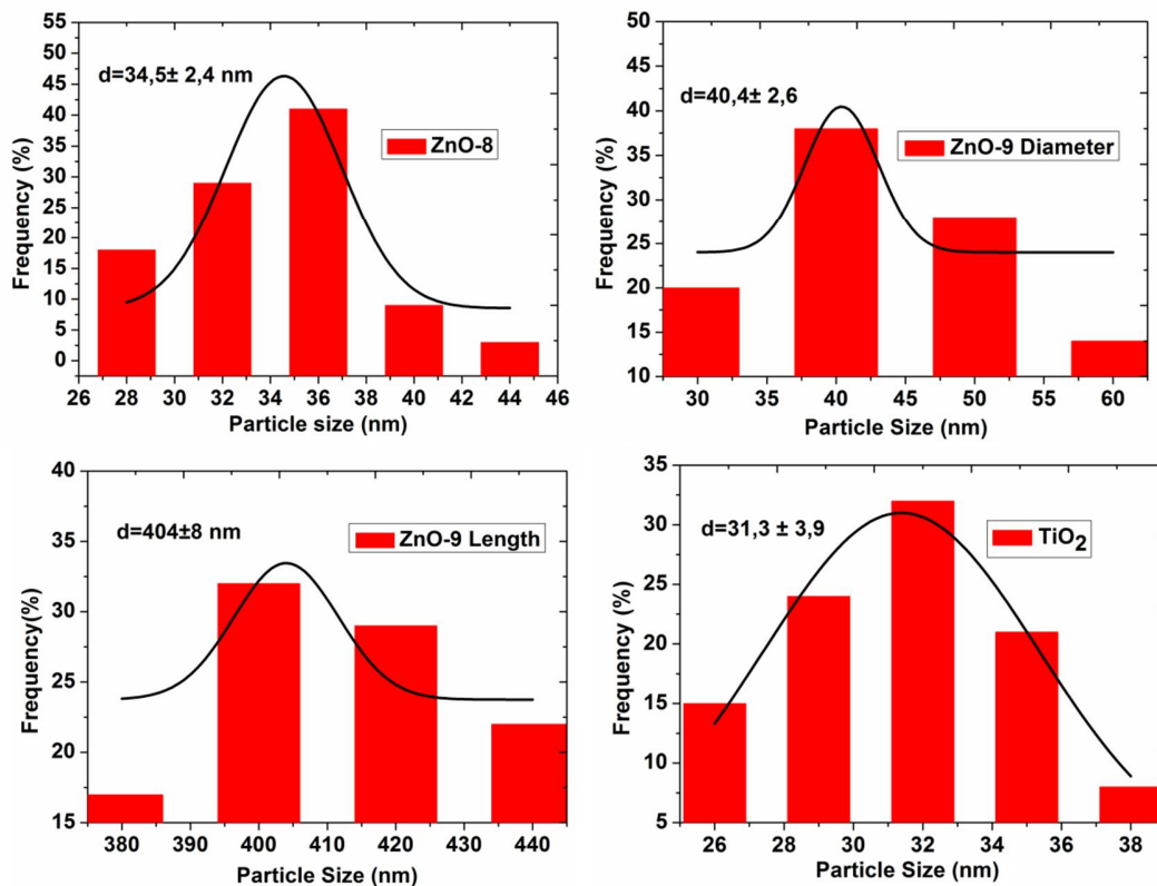
Figure S1. Size distribution charts of the ENs. Transmission electron microscopy (TEM) was used to investigate the size of the ENs. Hundred particles were counted for each sample. Size distribution charts presented show the particle size frequencies, an average diameter and a calculated statistical standard deviation acquired with non-linear fitting of the data for each sample.
