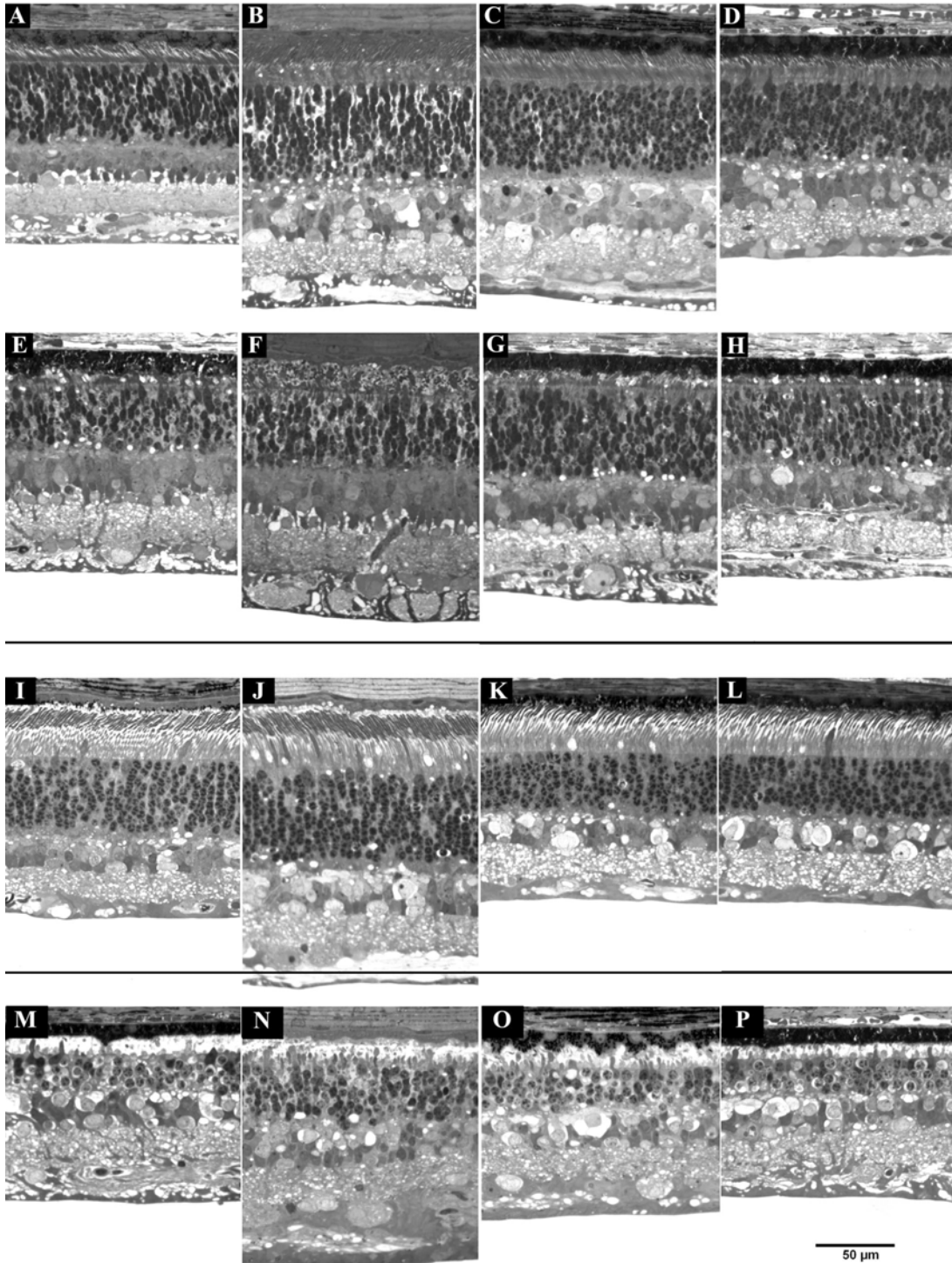
Supplemental Information Figure 1. Comparison of retinal histology at four different retinal regions (from left to right regions 2, 4, 5 and 7 – see Figure 1. Region 2 is dorsal peripheral, 4 is central tapetal, 5 is central non-tapetal and 7 is ventral peripheral). A-D a
