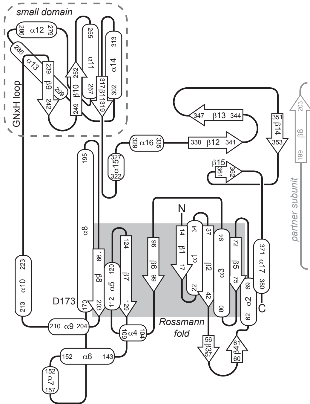
Figure S5. Topology diagram for H6YfdE.
