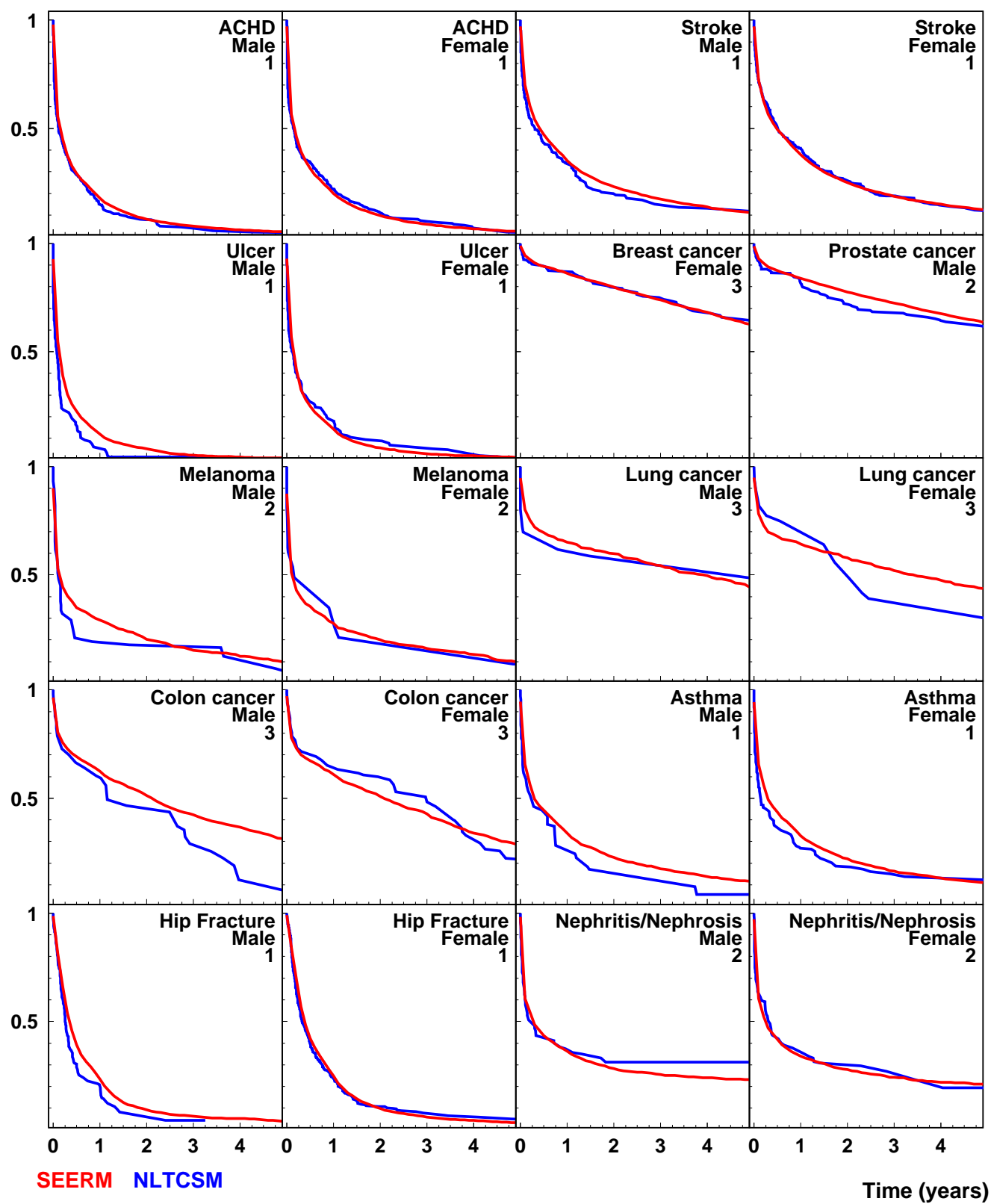
Supplemental Figure 1. The not-yet-recovery probabilities for selected recovery times calculated using SEER-M (red curves) and NLTCM-M (blue curves).
