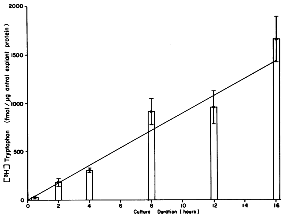
FIGURE 2 Incorporation of [ 3 H]tryptophan into tissue protein in cultured antral mucosal explants. The bars represent mean values for 4–12 experiments; the vertical lines indicate \pm 1 SEM. The solid line in this and subsequent figures represent a linear regression line.
