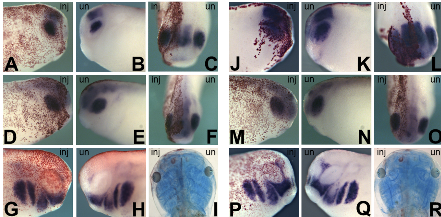
Figure S2. Results of antisense morpholino MoXat1 (A-I) or MoXat3 (J-R) injections in Xenopus embryos. Injections of 4 ng of single MO does not produce reduction in the expression of Xotx2 (A-C, J-L), nrp-1 (D-F; M-O) or Twist (G-H, P-Q) on the injected (inj) side of treated embryos compared to control (un) side. No reduction of pharyngeal skeleton is observed on the injected side in swimming larvae (I, R) compared to uninjected side. \beta -gal red staining traces injected side of embryos.
