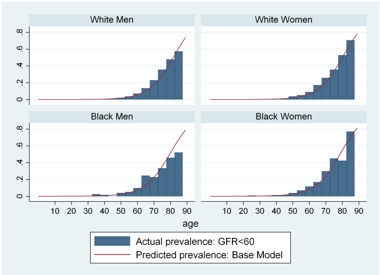
Figure S1. Actual versus predicted U.S. prevalence of CKD Stage 3a+, by age, sex, and race.
