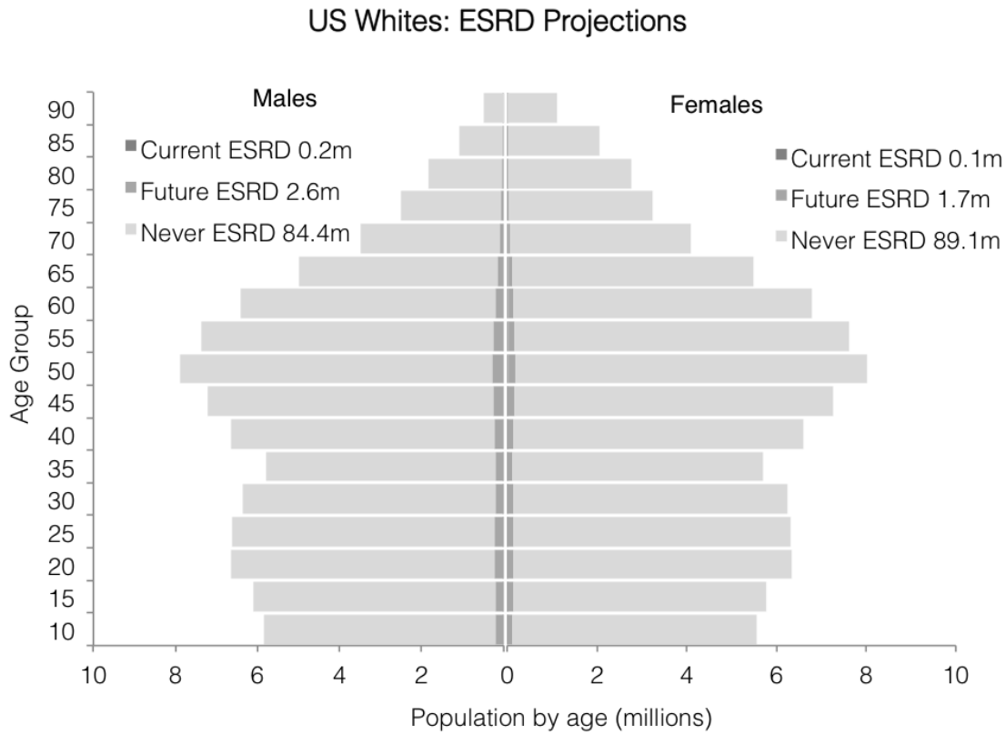
Figure S3. ESRD projections by age, race, and sex, scaled by estimated 2012 U.S. population
