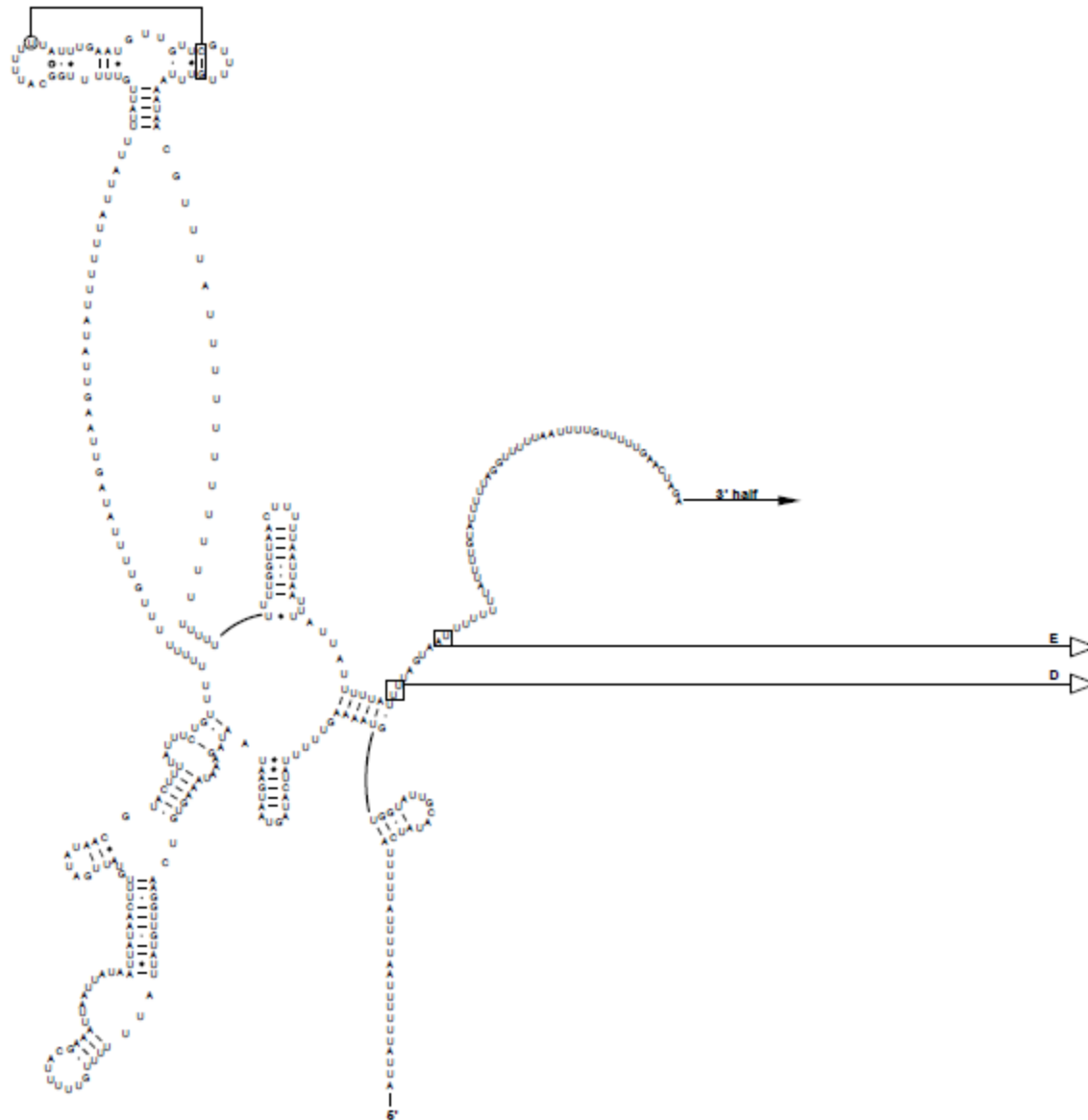
Figure S3c: Secondary Structure 5' half rrnL gene
