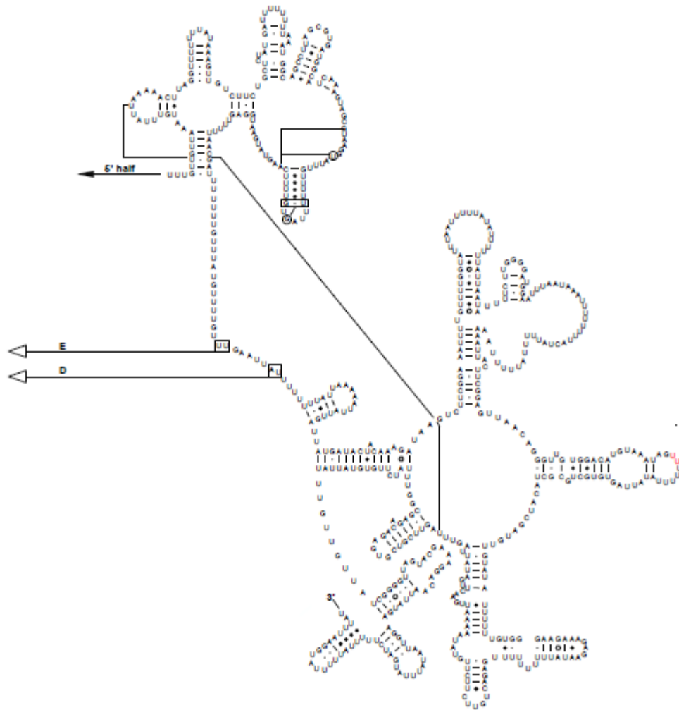
Figure S3b: Secondary Structure 3' half rrnL gene
