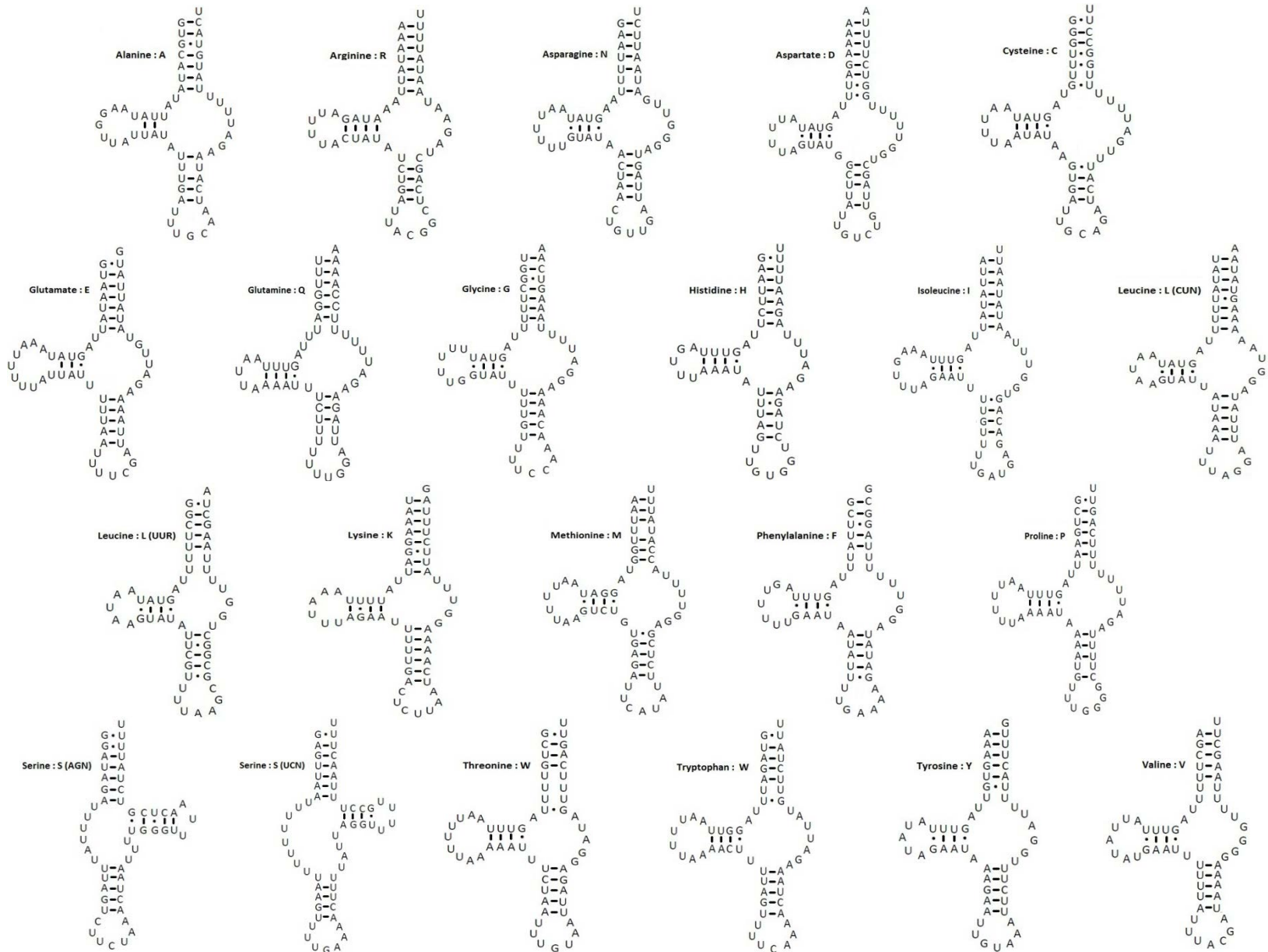
Figure S2: Predicted secondary structure of the 22 transfer RNA genes
