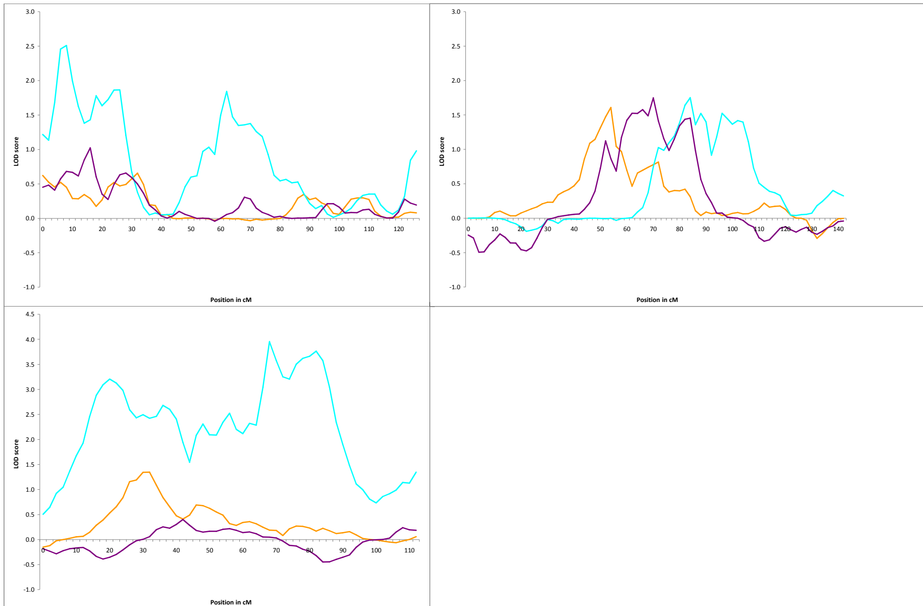
Figure S1. Linkage regions in the three geographically clusters at chromosome 14 (upper left panel), chromosome 17 (upper right panel) and chromosome 19 (lower panel). Light blue line represents Northern Europe cluster, orange line represents Southern Europe cluster, purple line represents Finland.
