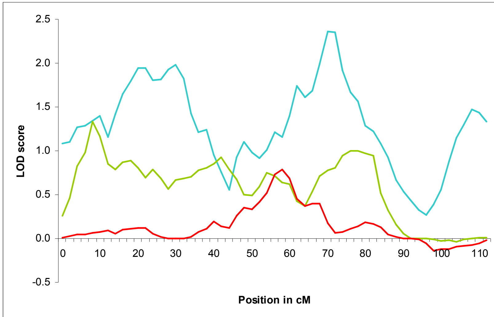
Figure S3. Linkage at chromosome 19 for the three largest centers from the Northern European cluster. Blue line represents Denmark, green line represents The Netherlands, red line represents France.
