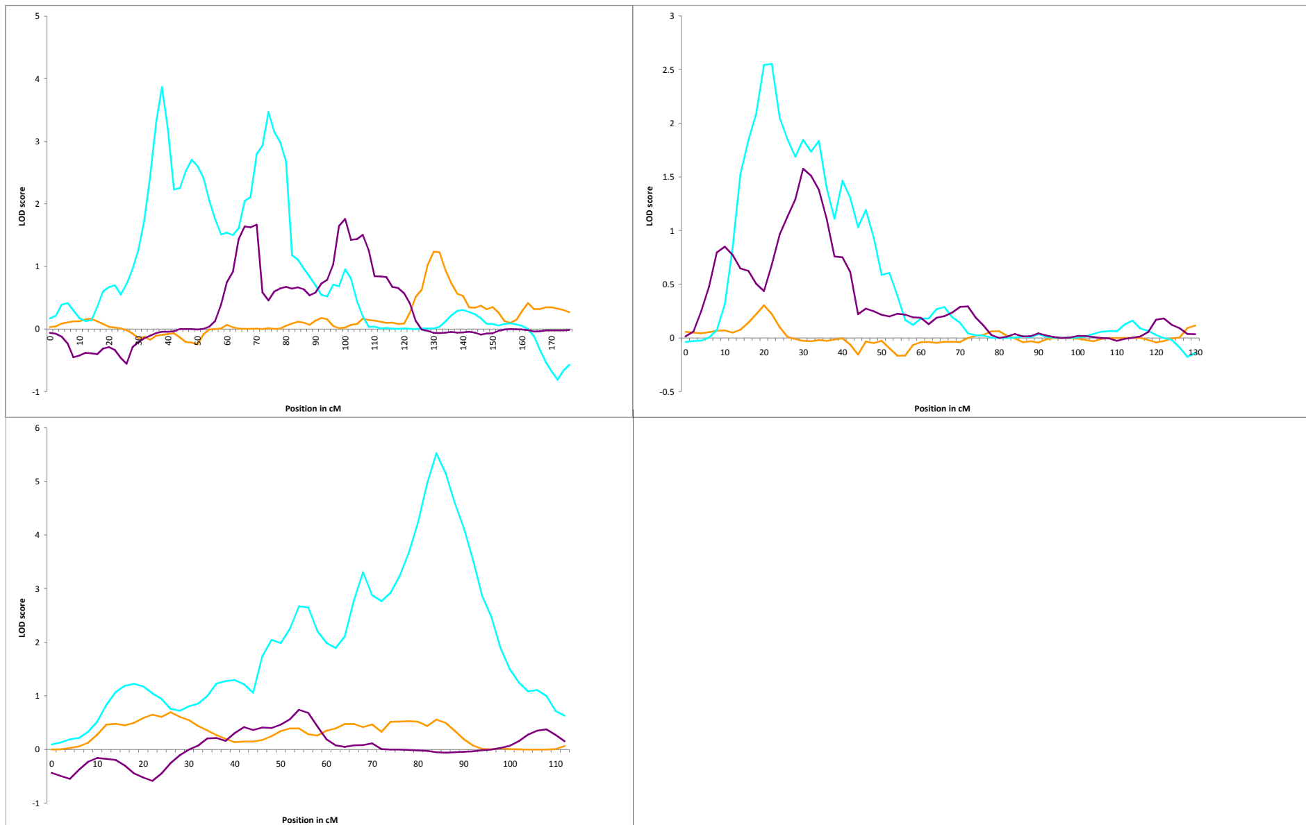
Figure S2. Sex-specific linkage regions in the three geographically clusters. Light blue line represents Northern Europe cluster, orange line represents Southern Europe cluster, purple line represents Finland. Left upper corner shows chromosome 8 in male-only sibpairs. Right upper corner shows chromosome 15 in female-only sibpairs. Left lower corner shows chromosome 19 in female-only sibpairs.
