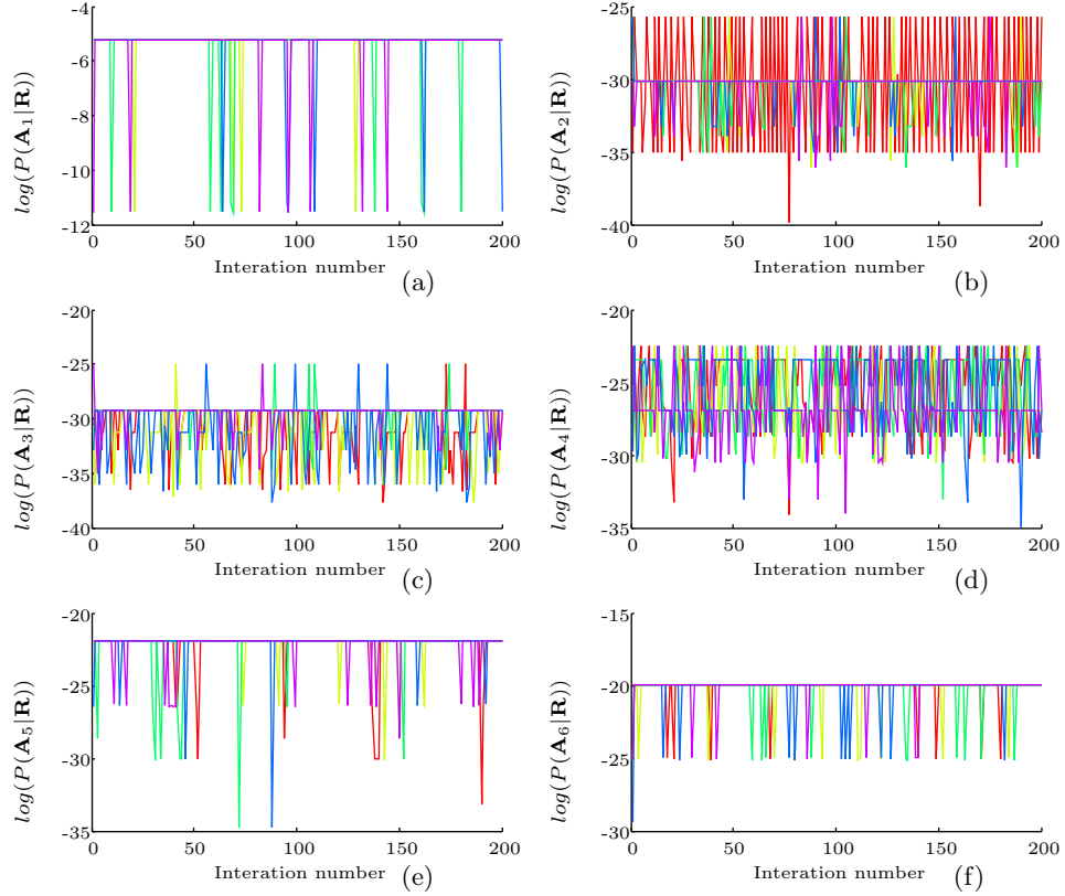
Figure S1: Convergence of the Gibbs samplers for noisy free data. The log-marginals of the samples are plotted in the Y-axis and the corresponding iteration numbers is plotted in X-axis. (a) shows the log-marginals of samples produced by 5 parallel samplers (indicated by five different colors) searching for the potential regulators of the receptor (EGFR) module. (b),(c),(d),(e) and (f) show the same for the adaptor (Grb2SOS), initiator(Ras), MAP3K(RAF), MAP2K(MEK) and MAPK(ERK) modules respectively. It can be noticed that in each subplot, the lines of different colors cover the same area in the plot, suggesting that the parallel samplers were sampling from the same distribution. If the samplers were sampling from different distribution one would expect the lines of different colors not to overlap on each other.
