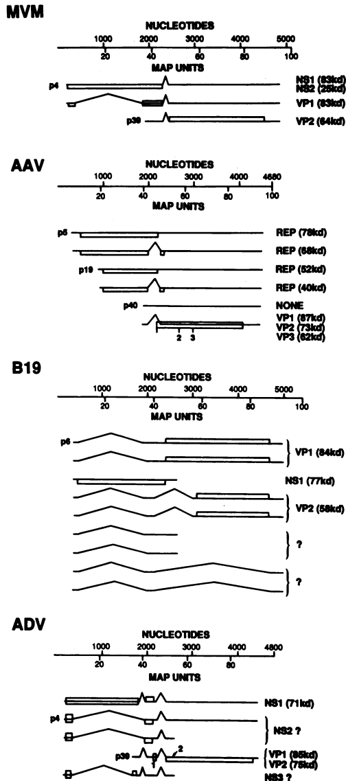
FIG. 1. Genetic and transcriptional maps of four representative parvovirus genomes. The RNAs illustrated are those detected by Northern blots or cDNA cloning. Symbol: □, open reading frames thought to be translated from each RNA. The position of the box relative to the transcript indicates the reading frame used: above, 1; straddling 2; below, 3. Known proteins and molecular masses (in kilodaltons [kd]) are indicated to the right (? indicates that the protein has not been observed). Map positions of promoters are to the left. Introns are indicated by interruptions in the RNAs. See text for details on closely spaced alternative splice donor and acceptor sites of MVM and AAV. Abbreviations: REP, AAV NS proteins; VP, virion structural proteins.
