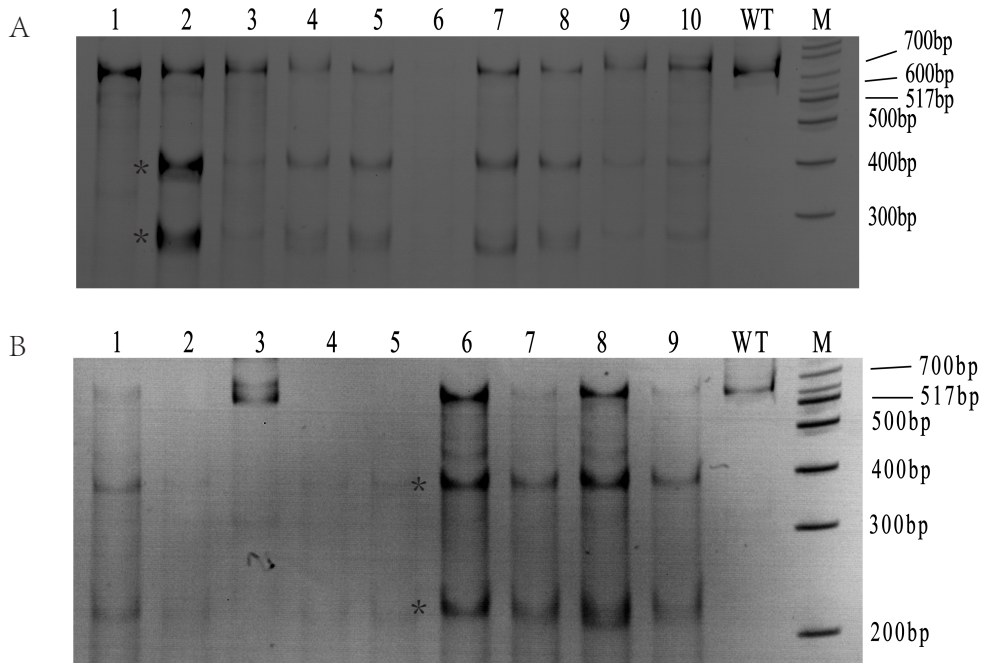
Figure S1 TALEN modification of RAG1 (A) and RAG2 (B) gene in in-vitro cultured rabbit blastocysts with T7 endonuclease I assay. The expected lengths of the T7E1 digestion products are indicated as “*”.
