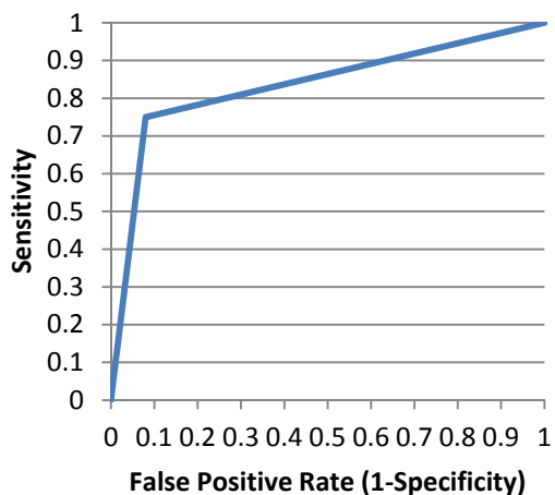
Validation Set, AUC = 0.84
