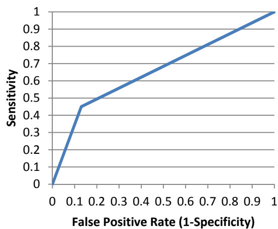
Test Set, AUC = 0.66
