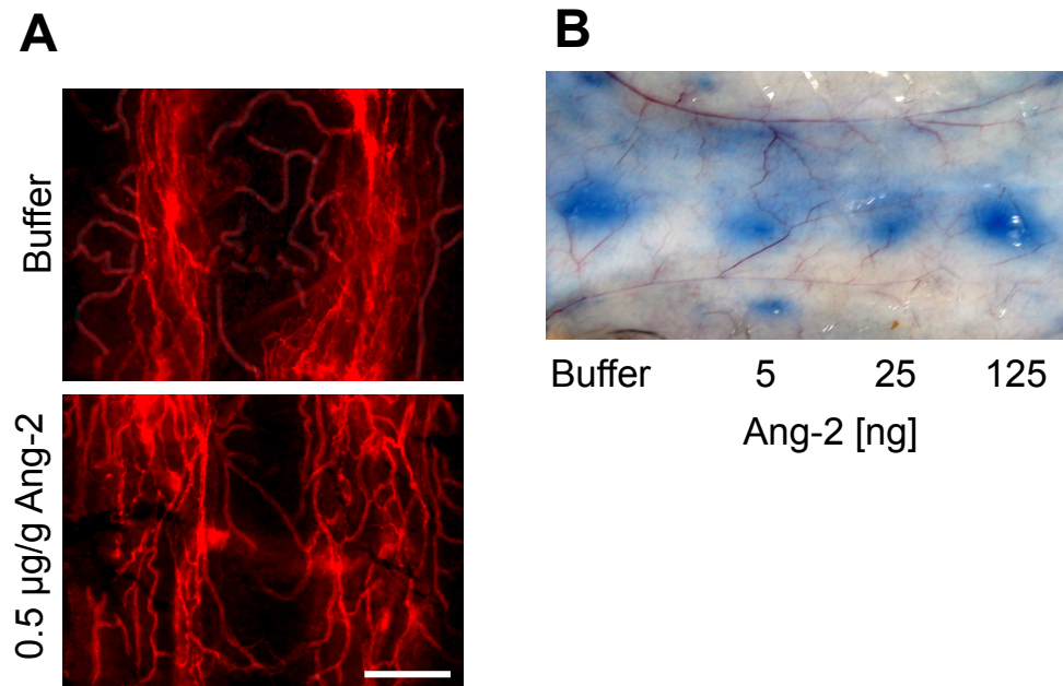
Supplementary Figure S3: Representative images of CD31-stained tracheal vasculatures ( A ) and Miles' Assay ( B ) following rhAng-2 administration. Scale bar 100 \mu\text{m} .
