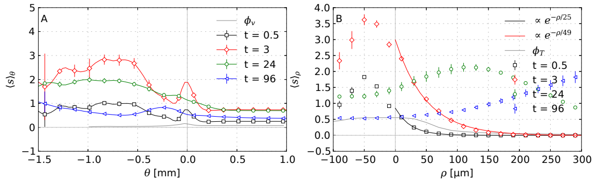
Figure 4: Drug concentration profiles at different times. (A) plotted vs. \theta , and (B) vs. distance from vessels \rho . Corresponds to Figure 8 in the paper.
