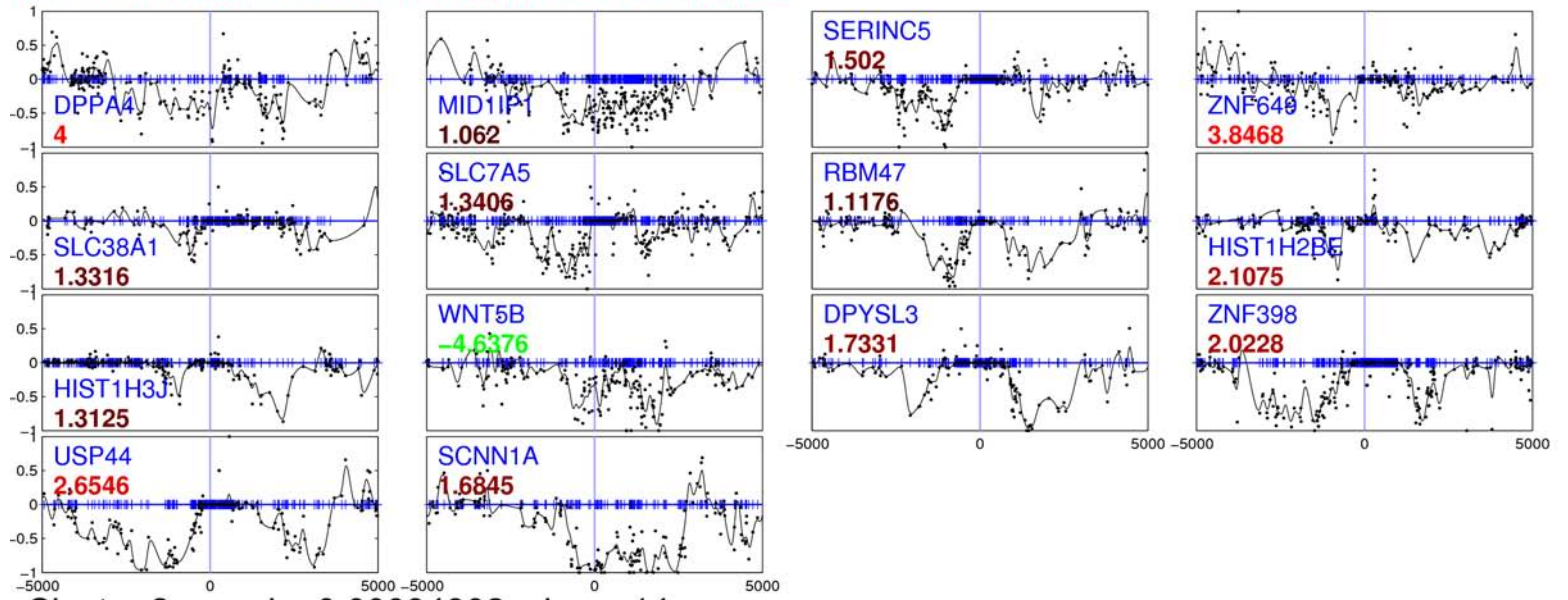
Cluster 2, pval = 0.00034302, size = 14
