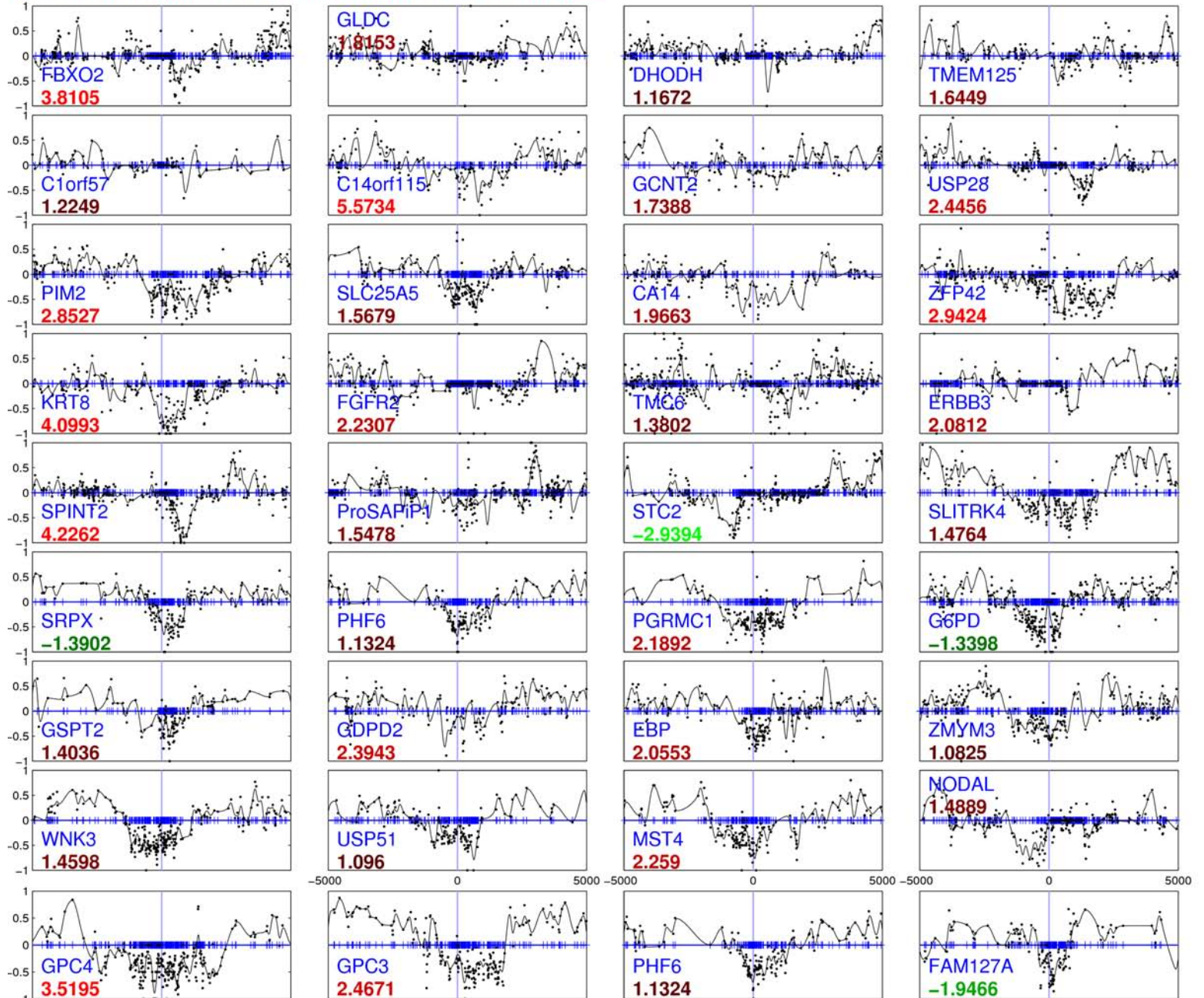
Cluster 4, pval = 0.00016892, size = 33
