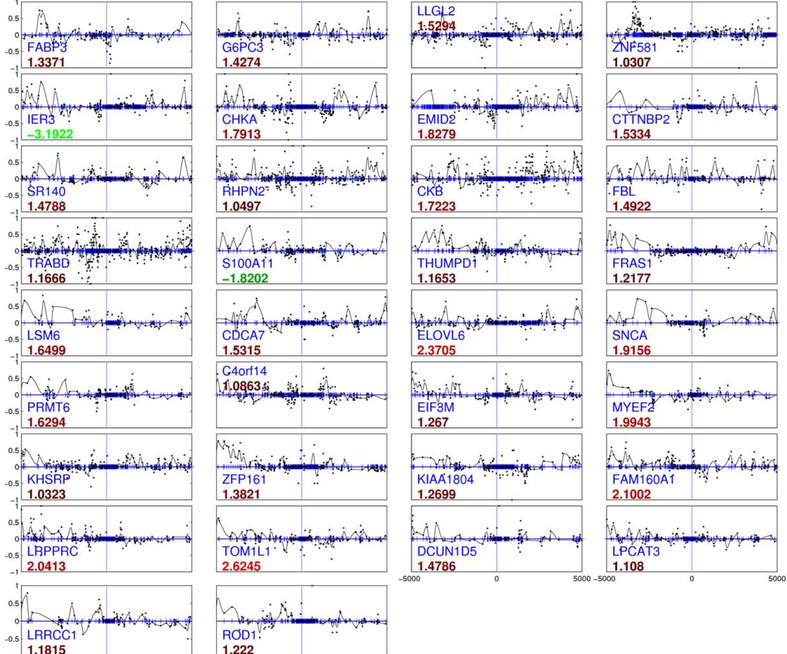
Cluster 1, pval = 7.4715e-05, size = 34
