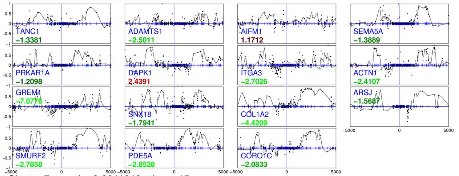
Cluster 7, pval = 0.0011819, size = 15
