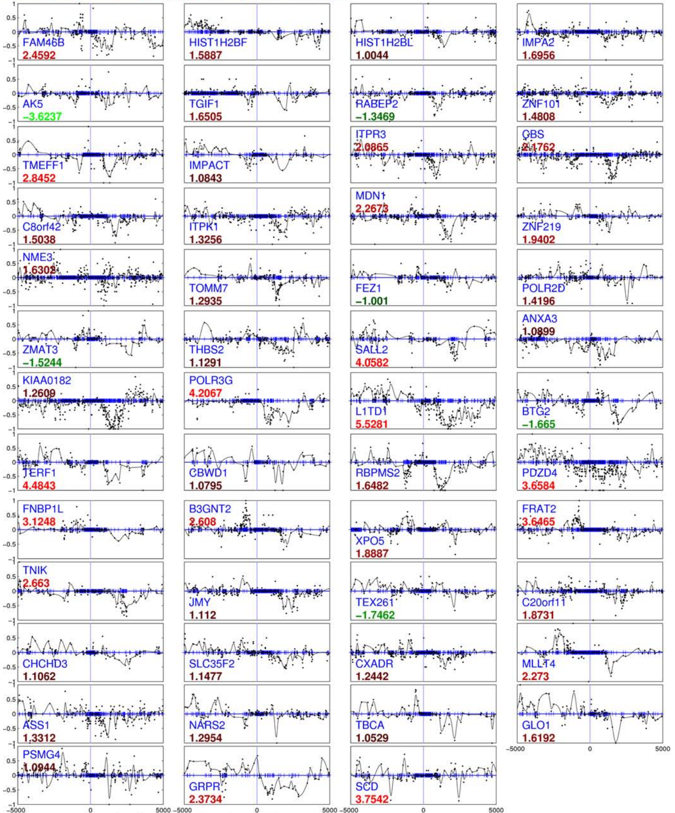
Cluster 5, pval = 0.0014176, size = 51
