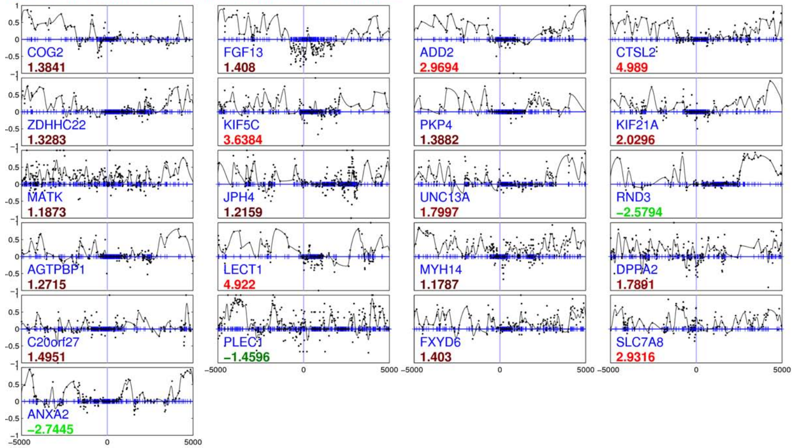
Cluster 10, pval = 7.4951e-05, size = 21
