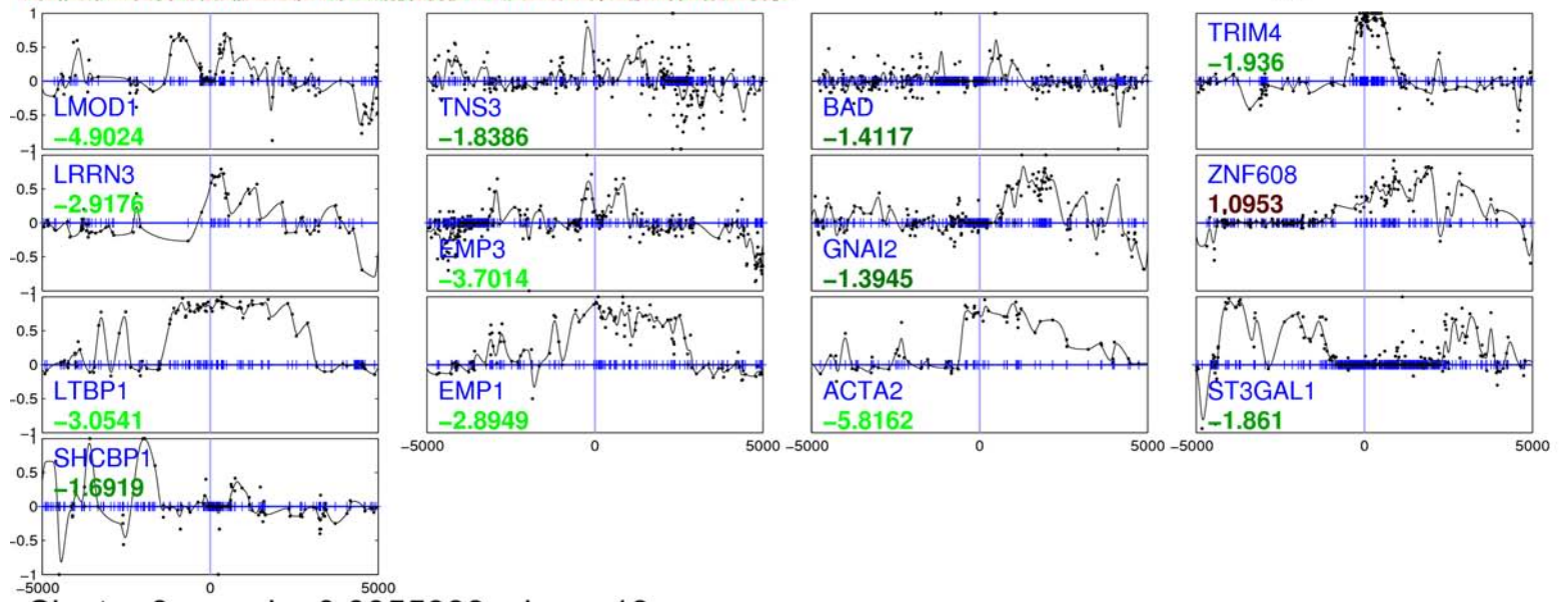
Cluster 3, pval = 0.0055933, size = 13
