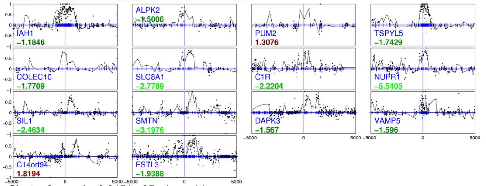
Cluster 8, pval = 9.3151e-05, size = 14
