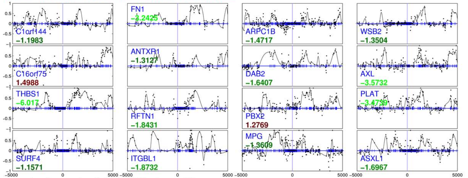
Cluster 6, pval = 0.0092535, size = 16
