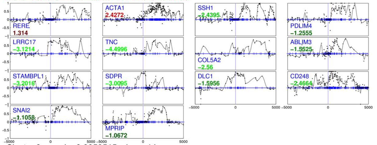
Cluster 9, pval = 0.0050515, size = 14
