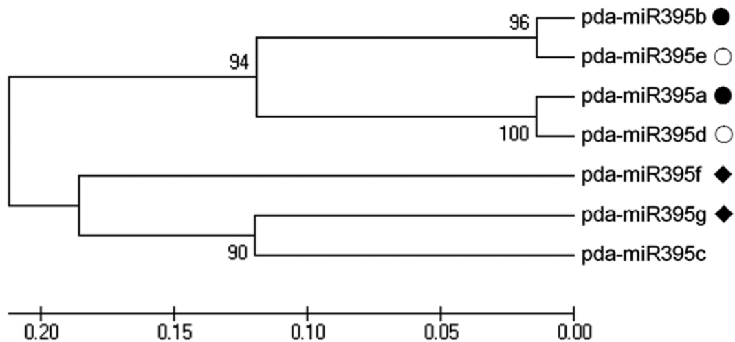
Figure S2. Phylogenetic analysis of microRNA395 pre-miRNAs in date palm ( Phoenix dactylifera ). Phylogenetic tree was formed by Neighbor Joining. The same symbols (●, ○, ◆) on the left of the miRNAs represent pairs miRNAs belong to tandem duplications.
