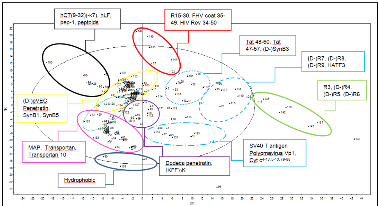
Figure S1. Score plot of the first versus the second principal component of the PCA-analysis of 186 peptides after dividing their descriptors by the molecular weight.
