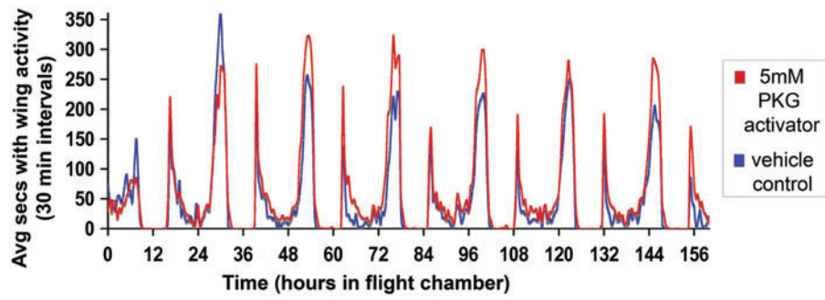
SUPPLEMENTARY FIG. S2. Aedes mosquitoes treated with protein kinase G (PKG) activator shows increased peaks of flight activity in morning and evening (run 3, with 5mM PKG activator).
