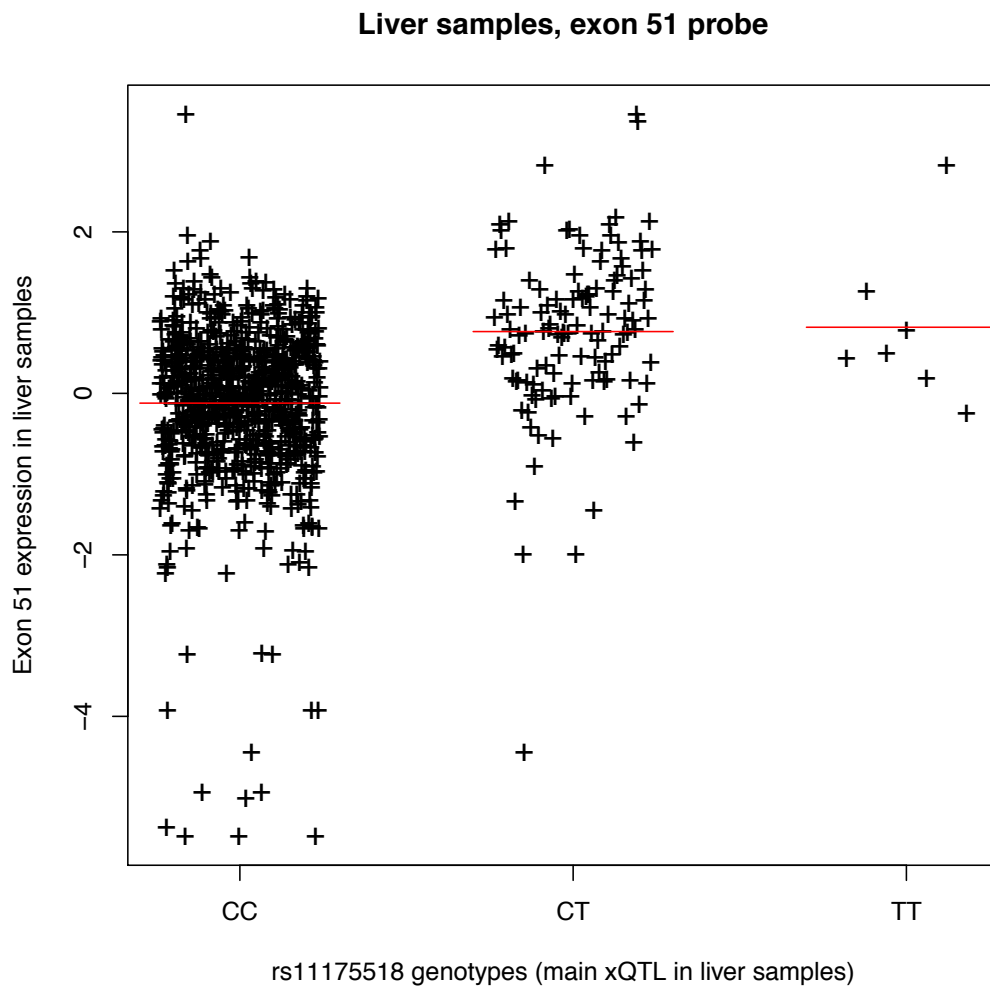
Figure S1: Expression-genotype correlation in 966 liver samples for the SNP rs11175518/exon 51 of LRRK2 .
