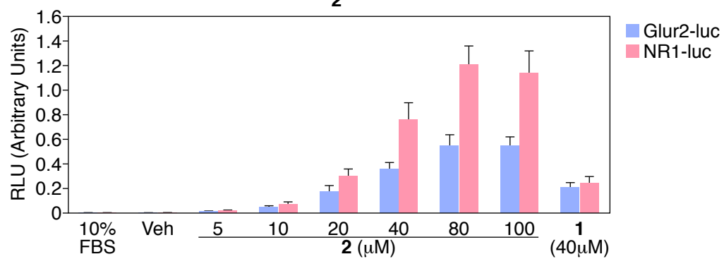
N-(5-hydroxypentyl)-5-(thiophen-2-yl)isoxazole-3-carboxamide 2
