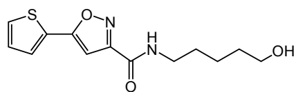
N-(5-hydroxypentyl)-5-(thiophen-2-yl)isoxazole-3-carboxamide 2
