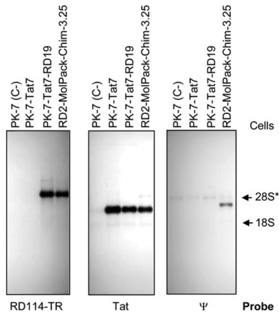
SUPPLEMENTARY FIG. S3. Northern blot analysis of the RD114-TR and Tat expression cassettes. Total RNA (5 \mu g/sample) derived from the different intermediate packaging and producer clones were hybridized with the specific probes as indicated. The size of the RD114-TR and Tat mRNA transcripts correspond to 4.9 and 2.6 kb, respectively. *Nonspecific hybridization of the 28S rRNA by the \Psi probe.
