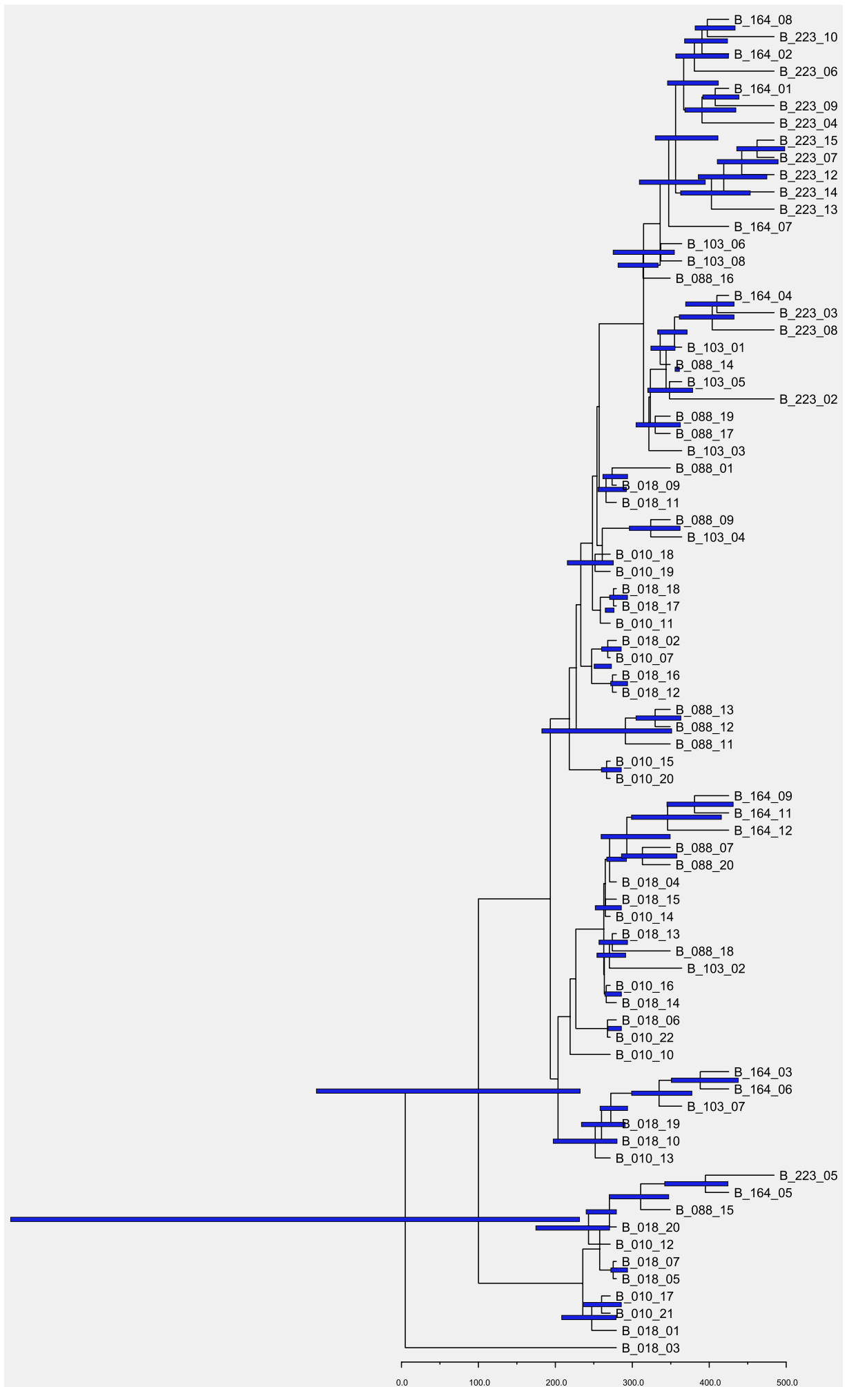
Figure S36 B-2865 env gp120 V1C5
