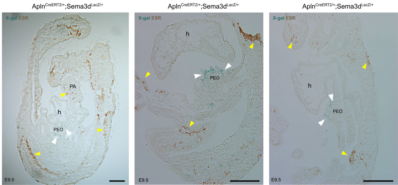
Supplementary information, Figure S4 X-gal and ESR double staining on E9.5 Apln^{CreERT2/+};Sema3d^{LacZ/+} embryos show no overlapping signal on proepicardial cells (PEO, white arrowheads). Yellow arrowheads denote the Apln^+ (ESR) cells in other region of embryos. black bar = 200 \mu m . PA, pharyngeal arch; h, heart; PEO, proepicardium.
