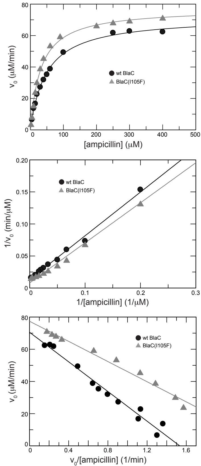
Supplemental Figure S3. Kinetics of wt and mutant BlaC enzymes. (a) Michaelis-Menten kinetics (top), Lineweaver-Burk plot (middle), and Eadie-Hofstee plot (bottom) generated for wt BlaC and BlaC(I105F) enzymes with Amp at single enzyme concentration (50 \mu\text{M} ).
