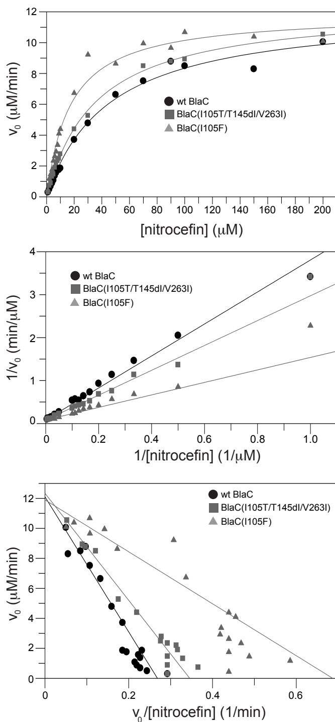
Supplemental Figure S4. Kinetics of wt and mutant BlaC enzymes. Michaelis-Menten kinetics (top), Lineweaver-Burk plot (middle), and Eadie-Hofstee plot (bottom) generated for wt BlaC and BlaC(I105F) enzymes with nitrocefin at single enzyme concentration (50 \mu\text{M} ).
