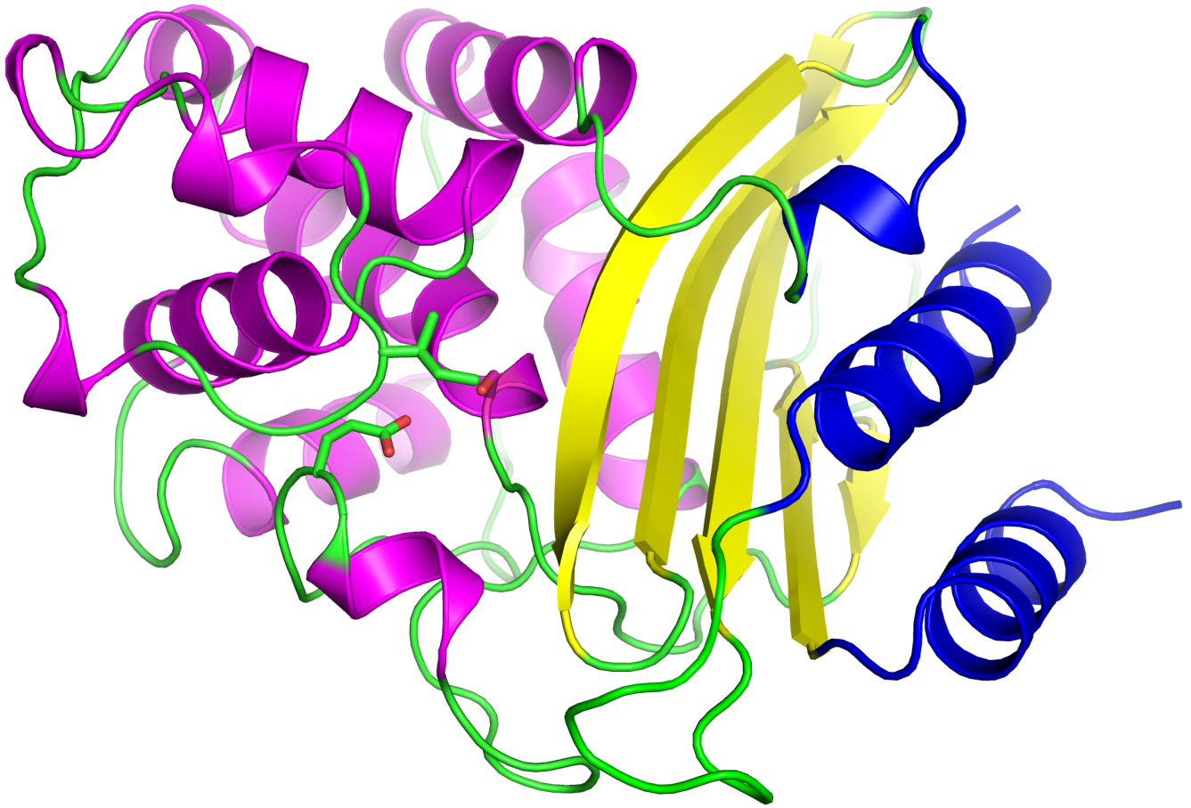
Supplemental Figure S6. Overall structure of full-length M. tuberculosis BlaC and its secondary structures. Clearly visible are the \alpha domain and an \alpha/\beta domain.
