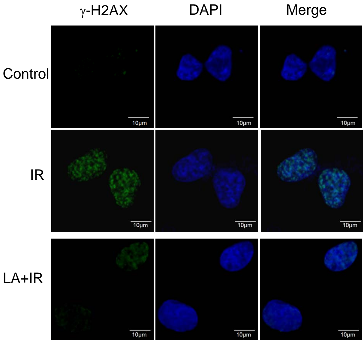
Supplementary figure 3. \gamma -H2AX foci formation was reduced in cells treated with Latrunculin A (1 \mu M) after IR (8Gy).
