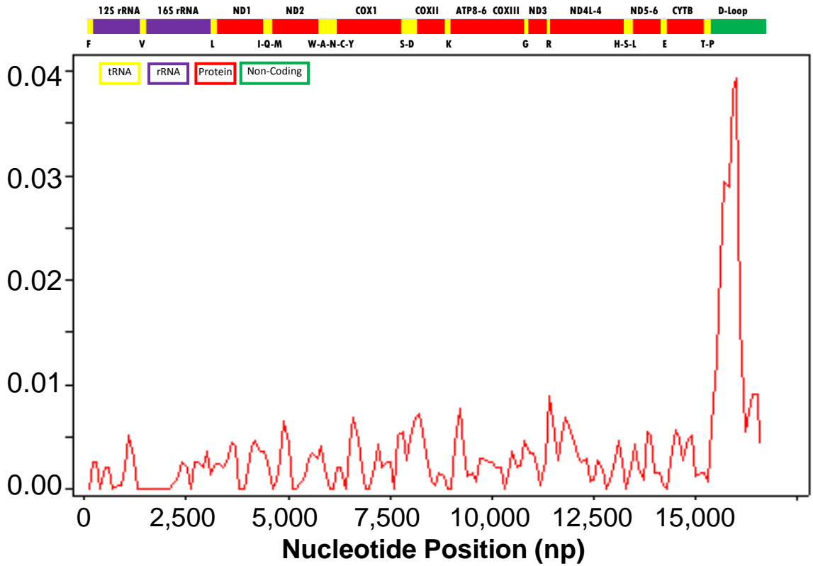
Figure S2. Nucleotide diversity variation ( \pi ) along the entire mitogenome.
