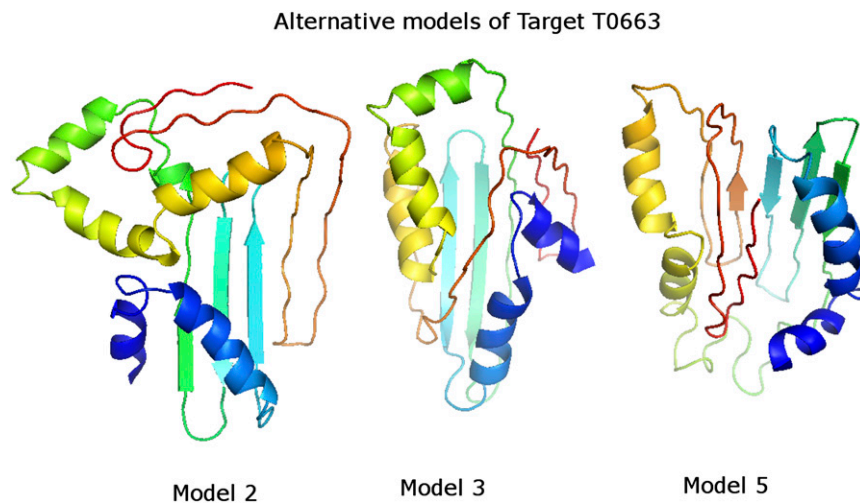
Fig. S1. Alternative models of target T0663 obtained with the United Residue force field in the 10th Community Wide Experiment on the Critical Assessment of Techniques for Protein Structure Prediction.
