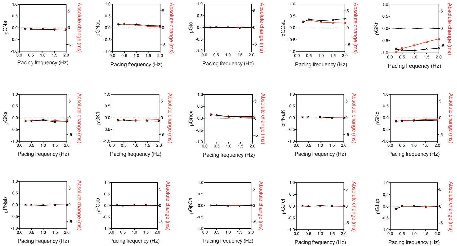
Supplementary Figure 3: Rate dependence of PLS regression coefficients ( \rho , black line) and absolute changes (red line) in QT interval for all ionic conductances in the ventricular cell model.
