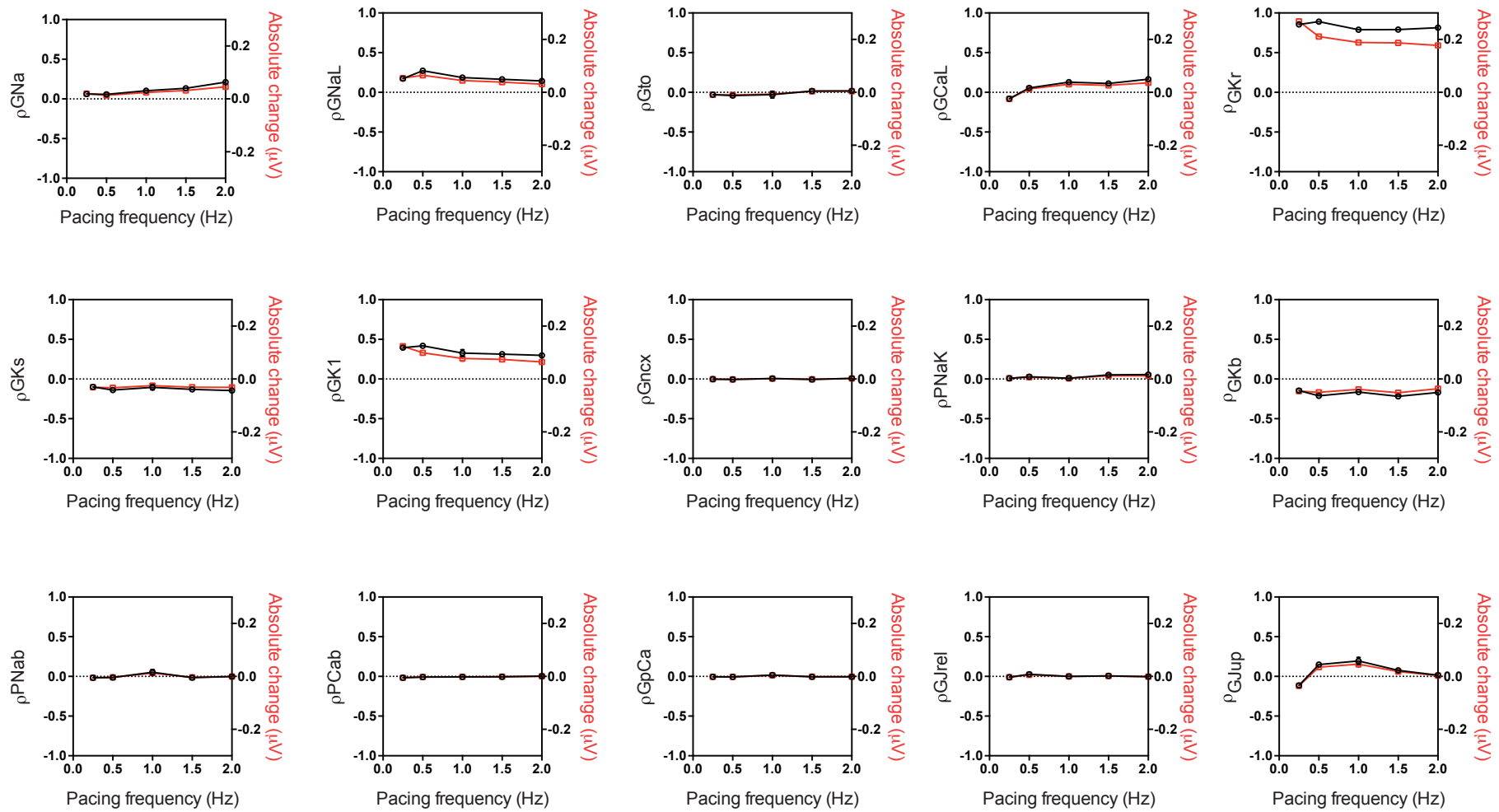
Supplementary Figure 5: Rate dependence of PLS regression coefficients ( \rho , black line) and absolute changes (red line) in T_{\text{height}} for all ionic conductances in the ventricular cell model.
