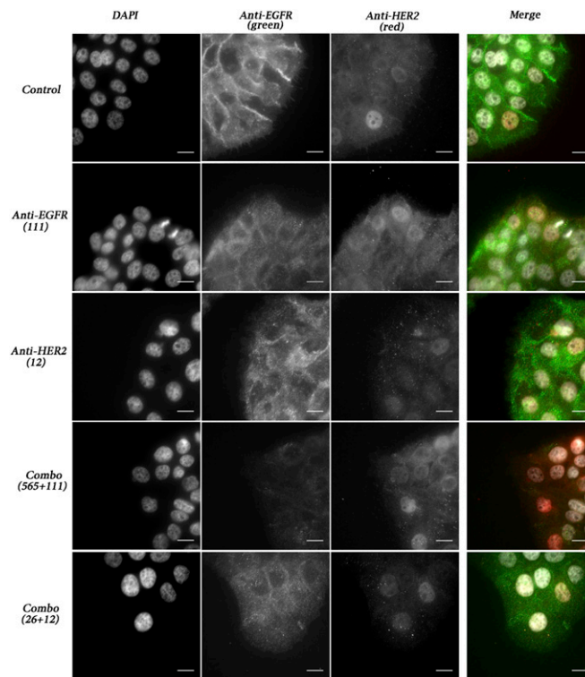
Fig. S1. Homocombinations of antibodies to epidermal growth factor receptor (EGFR) or to HER2 promote receptor down-regulation. BXP3 cells growing on fibronectin-coated coverslips were treated for 48 h with the indicated mAbs to EGFR (111 and 565) or to HER2 (12 and 26), either singly or in combination. Thereafter, cells were washed, permeabilized, and fixed. Shown are the results of staining with antibodies to EGFR (green) and HER2 (red), as well as counterstaining with DAPI.
